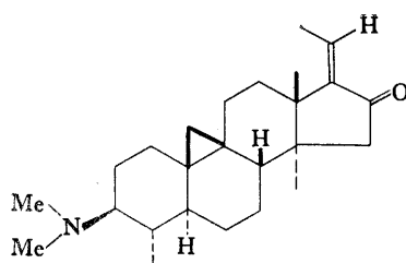
XVII Cyclobuxosuffrine
