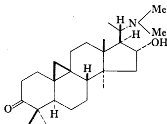
XXI Cyclomikuranine
