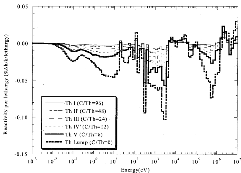
Figure 3.13 Energy dependence of reactivity difference caused by the use of different ^{232}\text{Th} cross sections, Case A.
