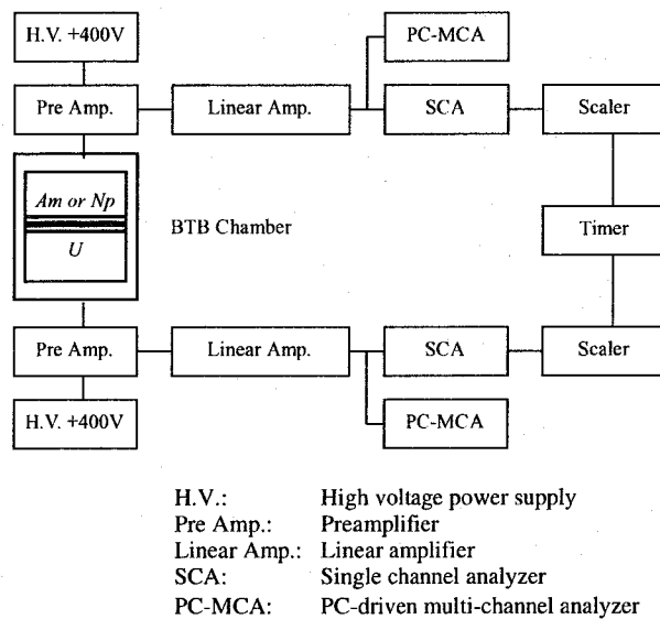
Figure 4.6 Electronic circuit.
