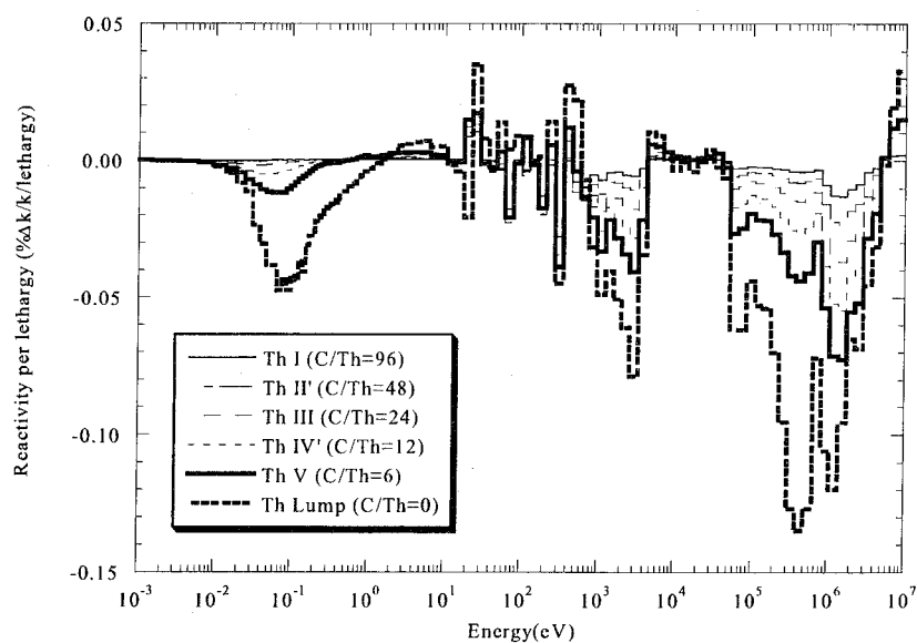
Figure 3.14 Energy dependence of reactivity difference caused by the use of different ^{232}\text{Th} cross sections, Case B.
