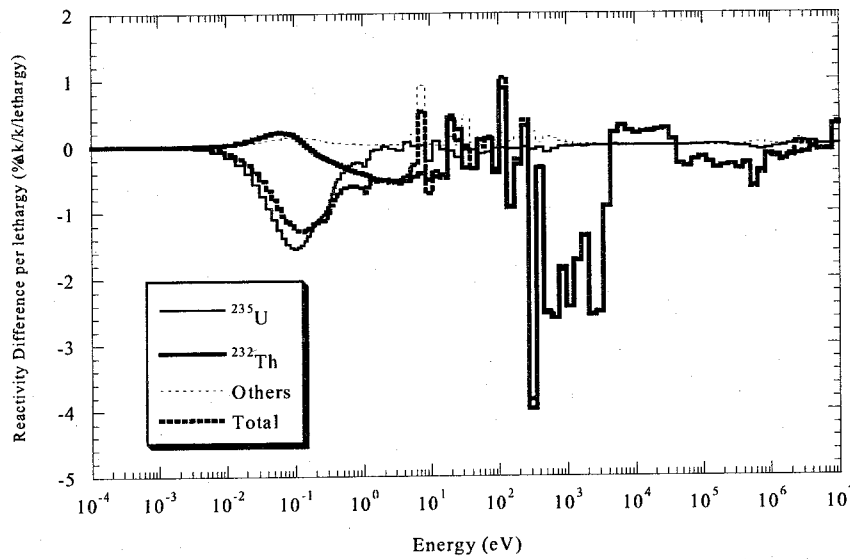
Figure 3.4 Breakdown of reactivity difference due to the use of different ^{232}\text{Th} cross sections in \text{ThO}_2\text{-UO}_2 Cell.
