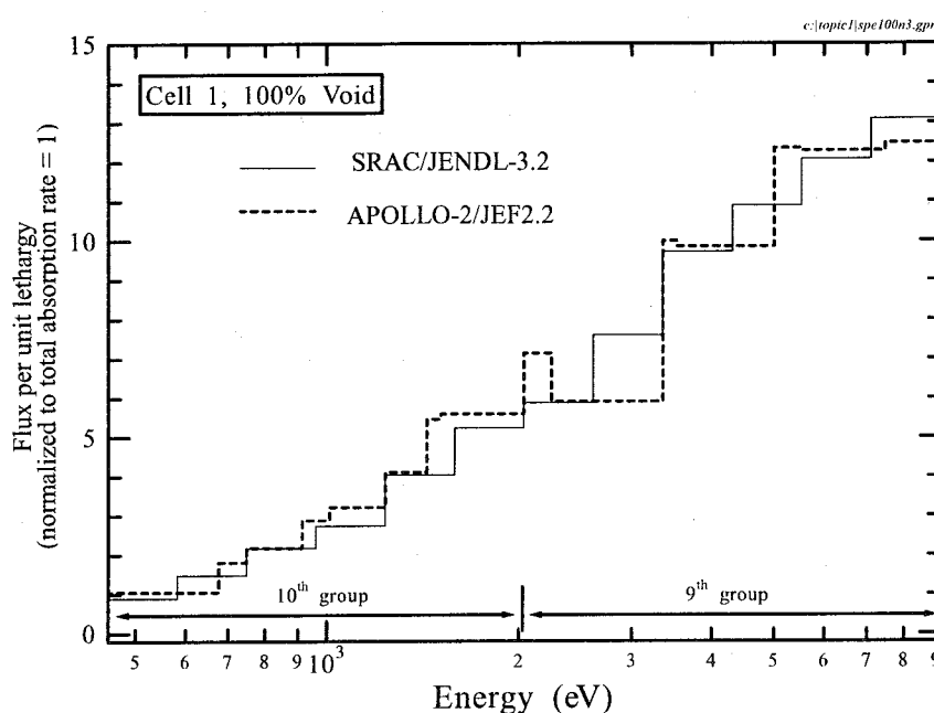
Figure 2.13 Comparison of cell-averaged neutron spectrum of Cell 1 at 100% void obtained by SRAC/JENDL-3.2 and APOLLO-2/JEF2.2. Energy range is 454 \text{ eV} < E < 9 \text{ keV} .
