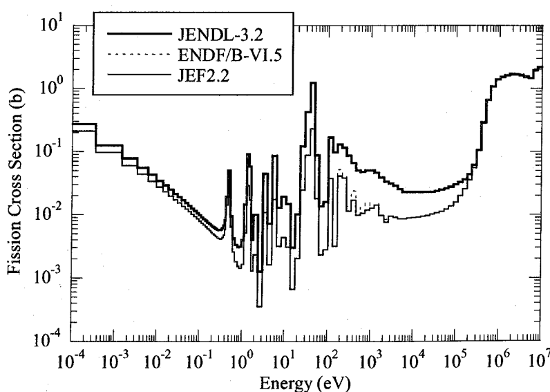
Figure 4.1 Fission cross sections of ^{237}\text{Np} .
