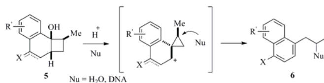
Scheme 2 Domino ring contraction-opening reaction of 5 in aqueous acidic conditions.
