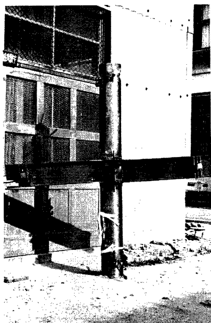
Photo. 10 PJHM after test.
