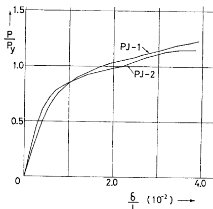
Fig. 13 Modified load-elongation curve of PJ-1 compared with that of PJ-2.
