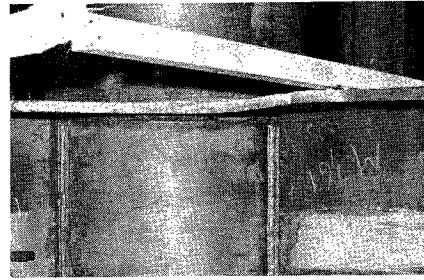
Photo. 9 Close-up of flange local buckling in PJVF.
