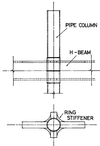
Fig. 1 Philosophy of “tension type” specimen.
