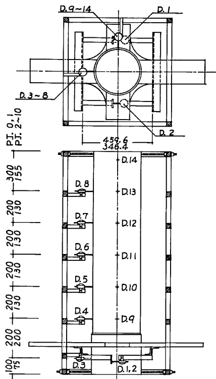
Fig. 11 Dial gage instrumentation for “tension type” testing.
