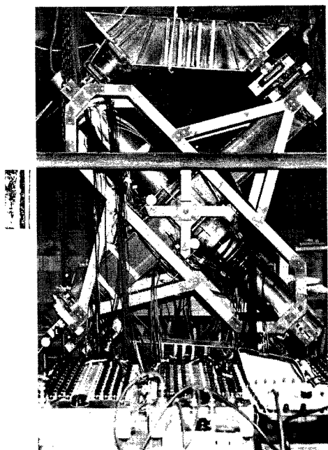
Photo. 3 Test set-up for "horizontal load type" testing (PJHM).
