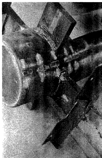
Photo. 6 Failure in "tension type" specimen PJ-2.
