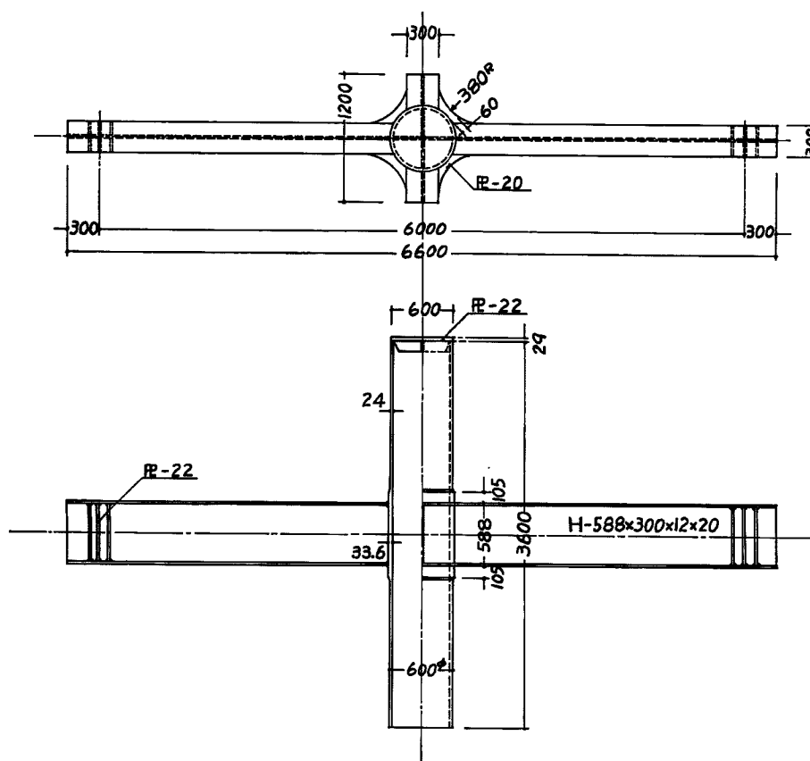
Fig. 4 Detail of full scale specimen—PJVF.
