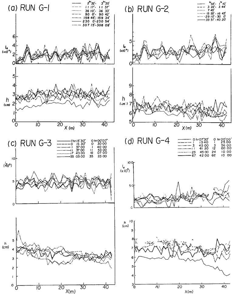
Fig. 3 Longitudinal changes of mean depth and energy slope in the experiments;
