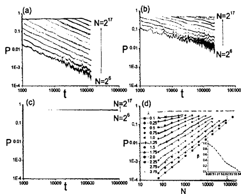
FIG. 2: Log-log plot of the survival probability P(t) at K = 0.3 and various \lambda (a) \lambda = 0.5 ; (b) \lambda = 1.5 ; (c) \lambda = 3.75 . In Fig. 2(d), P(N) \sim N^\beta for different \lambda at time t \sim 2 \times 10^5 . The inset of Fig. 2(d) shows \beta(\lambda) .
