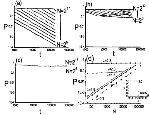
FIG. 1: Log-log plot of the survival probability P(t) at K = 0.15 and various \lambda (a) \lambda = 1.3 ; (b) \lambda = 2.2 ; (c) \lambda = 2.3 . In Fig. 1(d), P(N) \sim N^\beta for different \lambda at time t \sim 2 \times 10^5 . The inset of Fig. 1(d) shows \beta(\lambda) .
