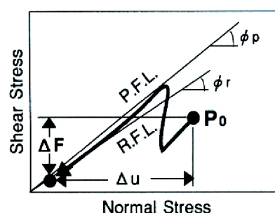
Fig. 8 Stress path and illustration of mass liquefaction (A) and the sliding-surface liquefaction (B) R.F.L.: Residual failure line, P.F.L.: Peak failure line
