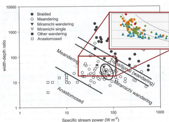
Fig. 1 RSCC in the Kizu River plotted in dimension of width/depth ratio and specific stream power (Burge, 2005). Kizu River was shown in meandering channel and transitional wandering channel.
