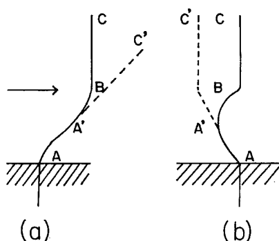
Fig. 15 Model graph of the rigid type slide (a) Flexion of the internal strain meter. (b) Accumulated strain graph.
