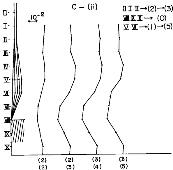
Fig. 8 Multiple sliding layer type (C-ii type).
