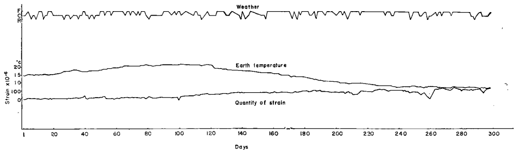
Fig. 22 Diurnal variation of strain ointernal strain meter at no strain state.
