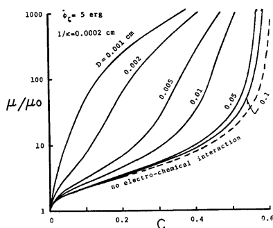
Fig. 10 Variation of relative viscosity by diameter
