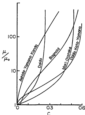
Fig. 6 Relation between relative viscosity and concentration
