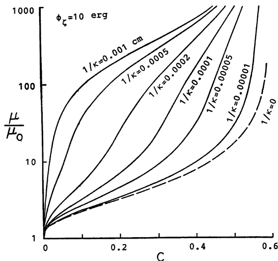
Fig 9 (c) Variation of relative viscosity by \phi_\zeta and \kappa
