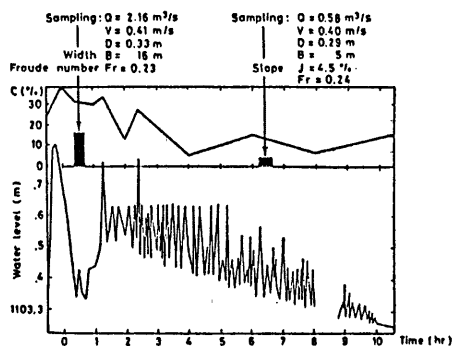
Fig. 4 An example of clogging phenomenon
