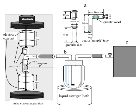
Fig. 1. Schematic of fast pyrolysis system 1
