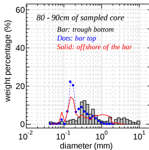
Fig. 7 Comparisons of grain size distribution
