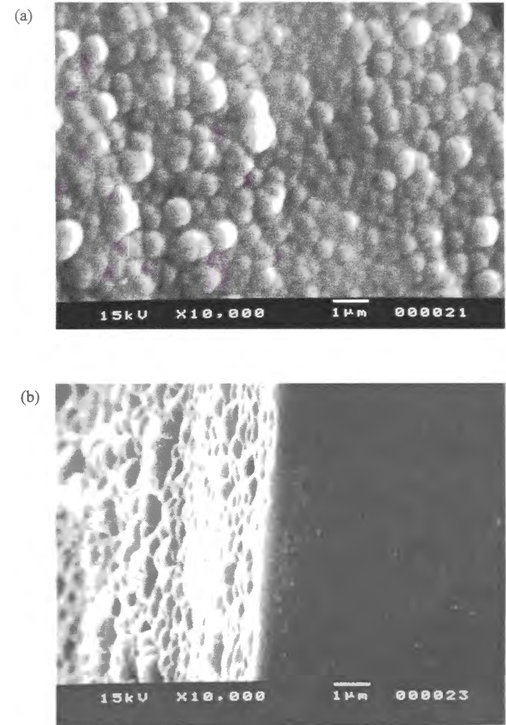
Fig. 8 SEM micrographs showing the membrane prepared by the CVD: (a) the outer surface and (b) the fractured surface.
