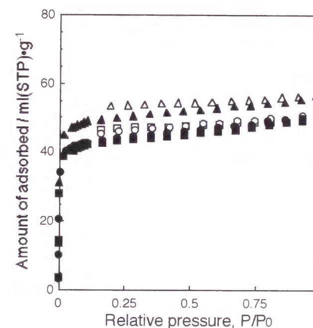
Fig. 5 N_2 adsorption-desorption isotherms of Al-0 glass hollow fiber membranes treated with 3 mol/dm 3 HNO 3 (○), H 3 PO 4 (Δ) and CH 3 COOH (□); solid symbols: adsorption, open symbols: desorption.
