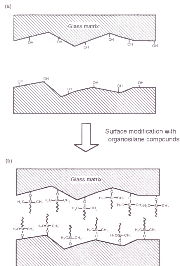
Fig. 14 Schematic representation of the pore structure of the surface modified membranes: (a) before surface modification, (b) after surface modification.
