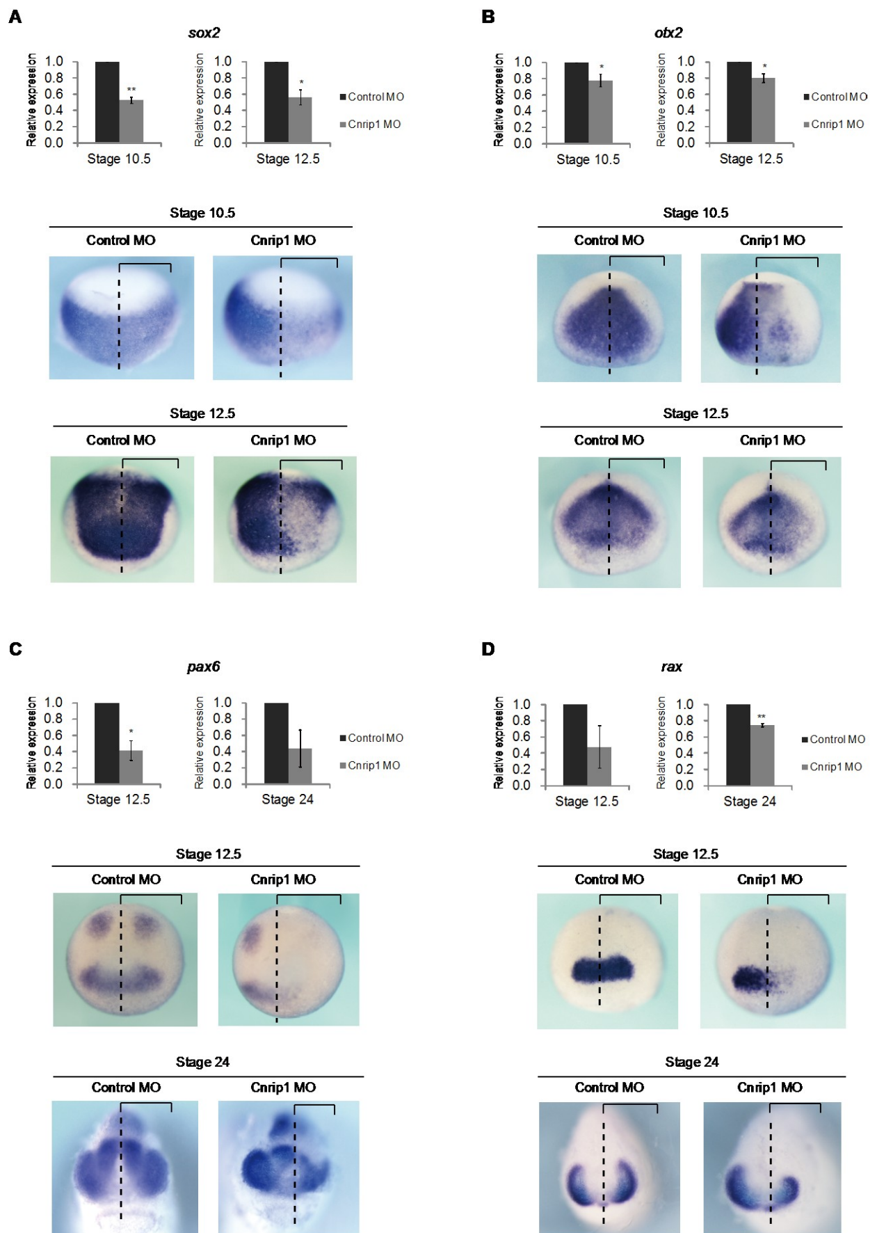
Figure 5. cnrip1 knockdown reduces the expression of sox2 , otx2 , pax6 and rax .
