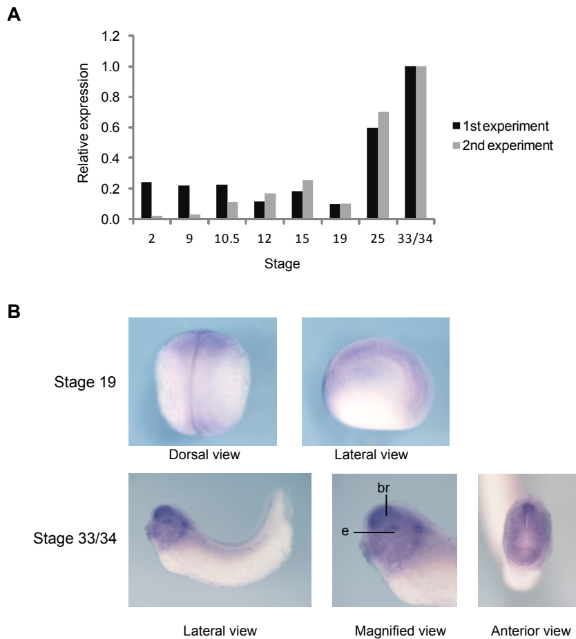
Figure 9. The expression pattern of Xenopus laevis cnr1 in early development.
