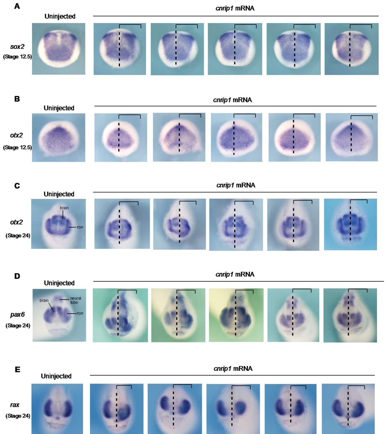
Figure 6. Effects of cnrip1 overexpression on the expression of sox2 , otx2 , pax6 and rax .
