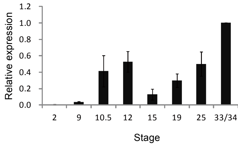
Figure 2. Temporal expression of cnrip1 in early Xenopus laevis development.
