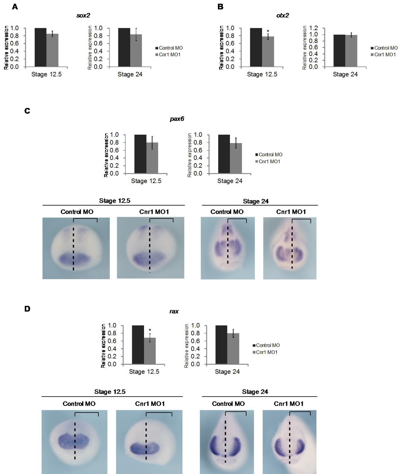
Figure 11. The effects of cnr1 knockdown on the expression of sox2 , otx2 , pax6 and rax .
