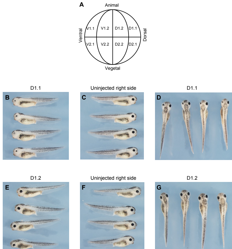
Figure 8. Knockdown of cnrip1 in the D1.1 blastomere causes eye and head defects.
