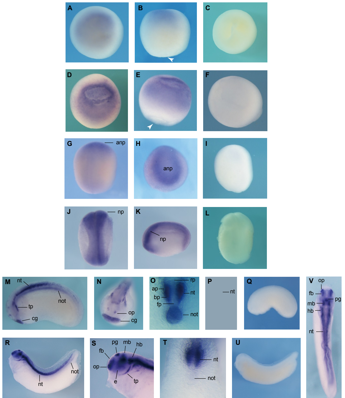
Figure 3. Spatial expression of cnrip1 in early Xenopus laevis development.
