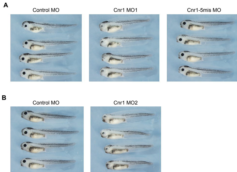
Figure 10. cnr1 knockdown leads to eye defects.
