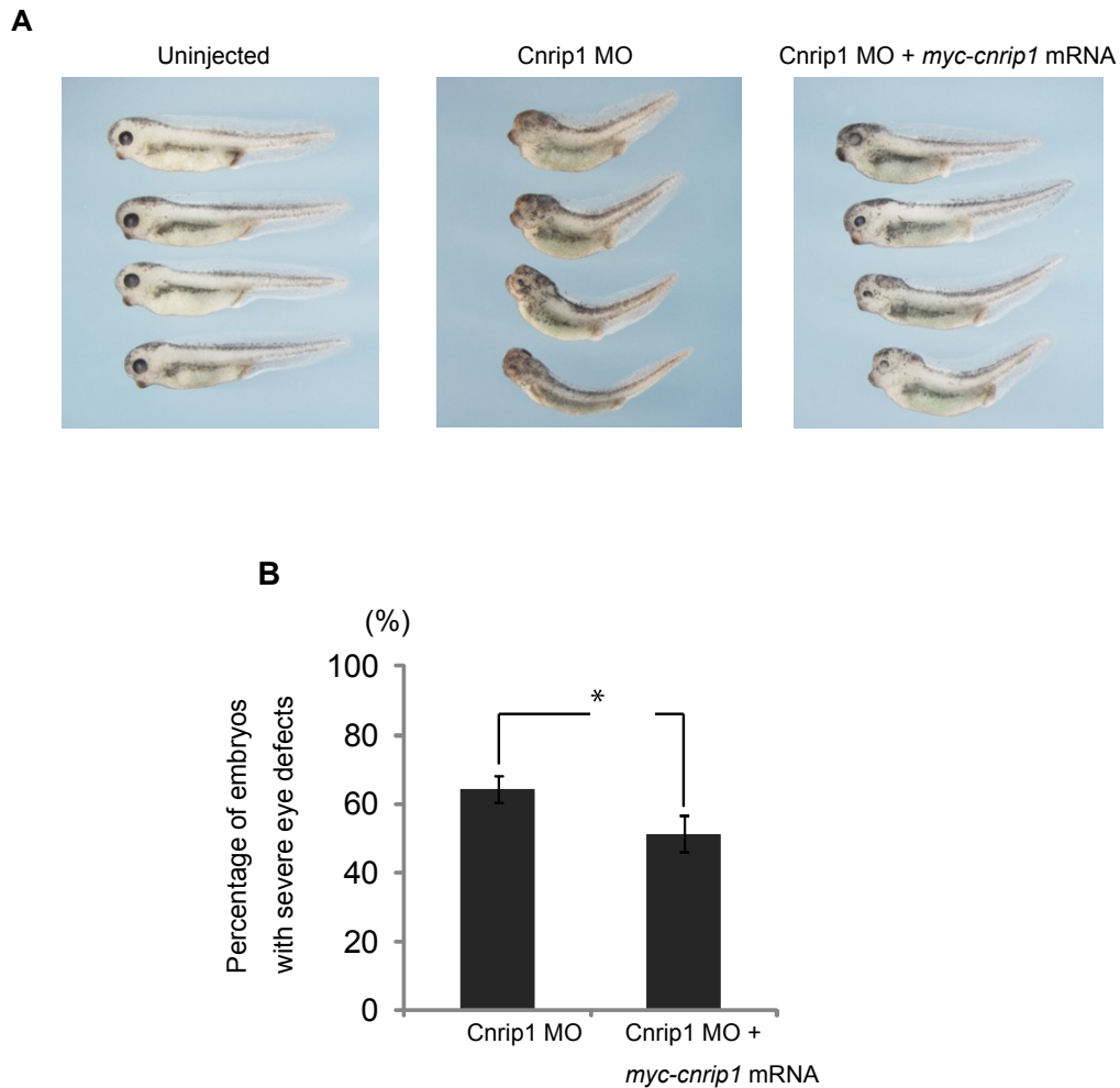
Figure 7. Partial rescue of eye development in cnrip1 knockdown embryos.
