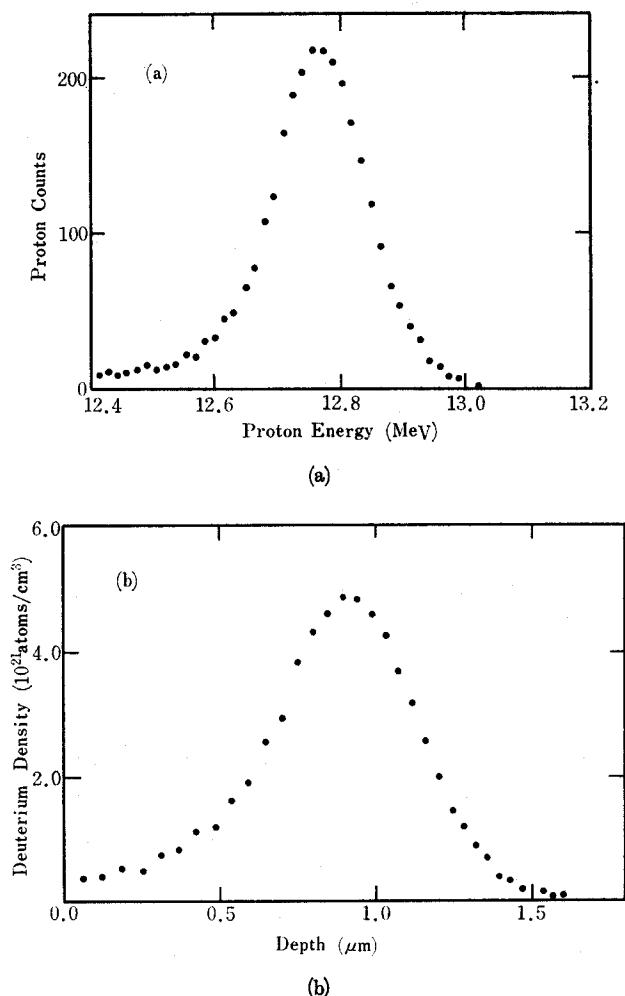
Fig. 4. An example of the results of depth profiling. (a) is plotted on an energy scale and (b) on a depth scale. (D-implantation: 1 \times 10^{17} cm -2 at 100 keV, 3 He energy: 1.1 MeV, Polishing: A.)
