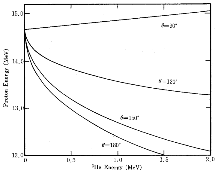
Fig. 2. Relation between emitted proton energy and incident ^3\text{He} energy at laboratory emission angles.
