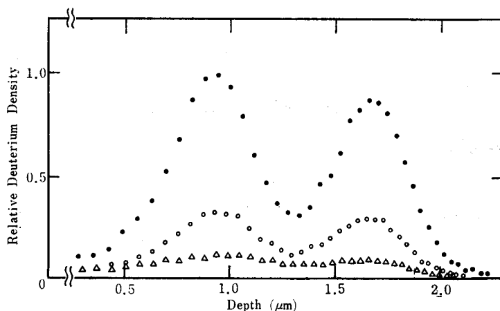
Fig. 7. Effect of annealing at 0^\circ\text{C} on the depth profile in double-implanted sample. ( D -implantation: 1 \times 10^{17} \text{ cm}^{-2} at 100 and 200 keV, ^3\text{He} energy: 1.3 MeV, ●: Before annealing, ○: Annealed for 2hr, △: Annealed for (2+6)hr, polishing: B.)
