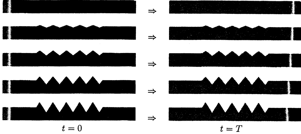
FIGURE 1. Numerical simulations of front propagation for (1.2) in five different domains when \varepsilon = 0.050 , f(u) = u(1-u)(u-1/4) . The white region approximately represents the position of the front.
