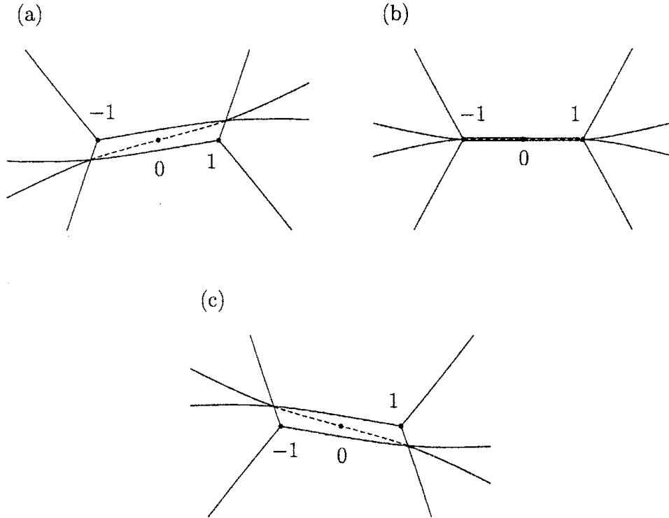
Figure 4 : Stokes geometry of (25) for (a) \arg \eta = (\frac{1}{2} - \frac{1}{12}) \pi , (b) \arg \eta = \frac{1}{2} \pi and (c) \arg \eta = (\frac{1}{2} + \frac{1}{12}) \pi .
