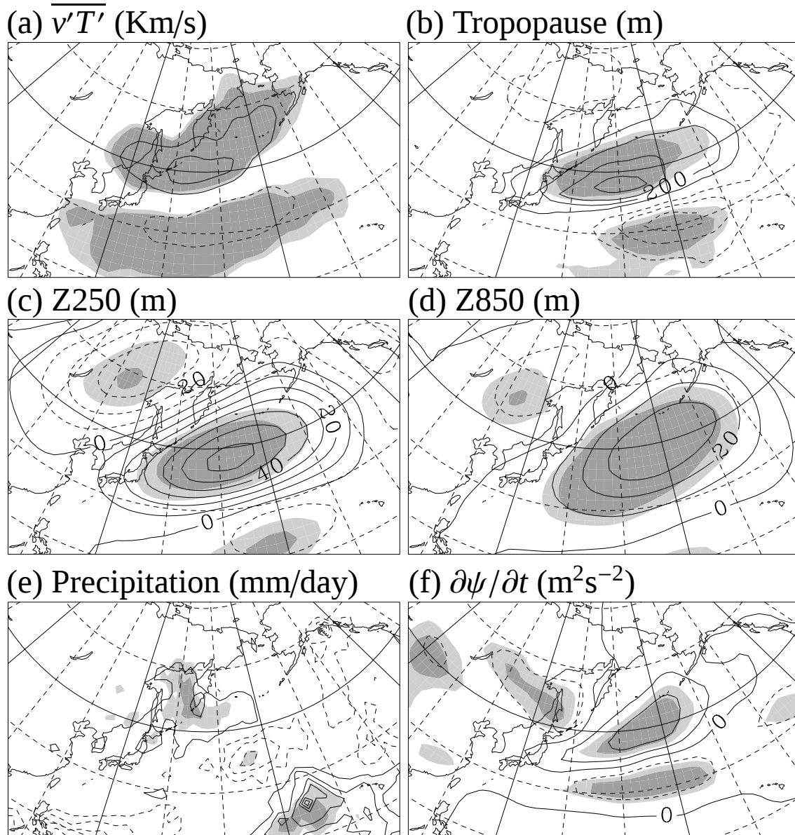
Fig. 4 As in Fig. 3, except for the anomalies associated with the PC2 LFV of the North Pacific storm track.
