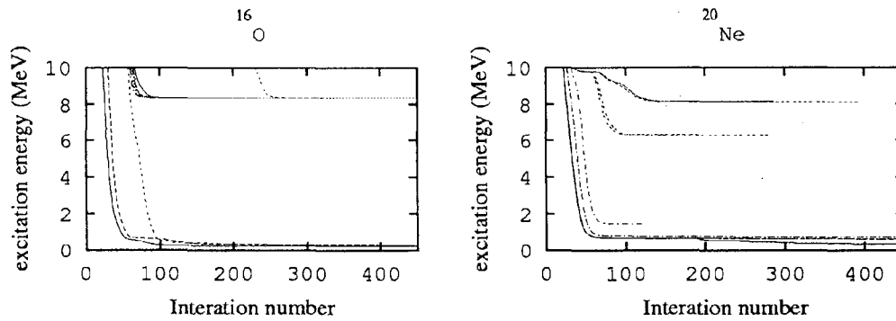
Fig. 1. Excitation energies of the nuclei ^{16}\text{O} and ^{20}\text{Ne} in the nuclear mean-field model with simplified interaction. Convergence of excitation energies is plotted against the iteration number in the conjugate gradient method.
