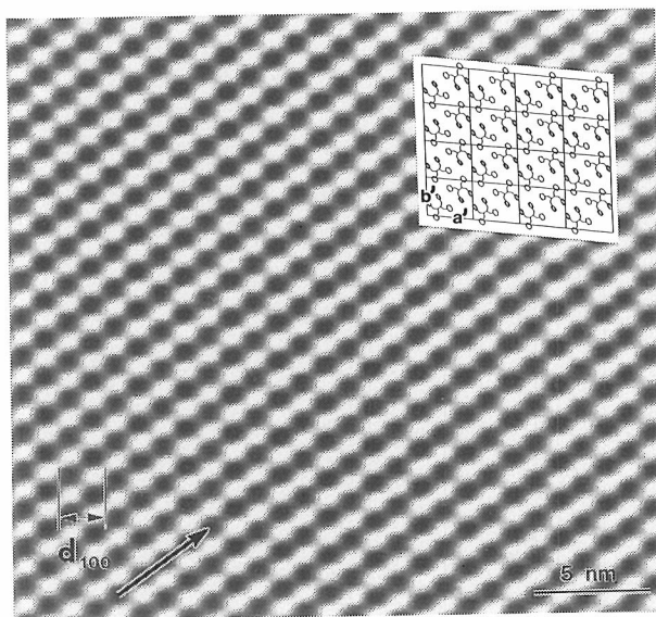
Fig. 8 Array of molecular images of PBPP \alpha -form, which were obtained from Fig. 7 by computer Fourier filtering 24) . Each dark dot corresponds to the PBPP molecular stem viewed along its axis. The inset is a model structure 23) : a'=1.66\text{nm} , b'=1.38\text{nm} , and the angle \gamma' between a' and b' axes is 97^\circ . The arrow indicates the direction parallel to the (1\bar{1}0) lattice plane.
