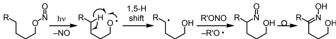
Scheme 3.12. Intermolecular radical reactions for carbon–nitrogen bond formation.
