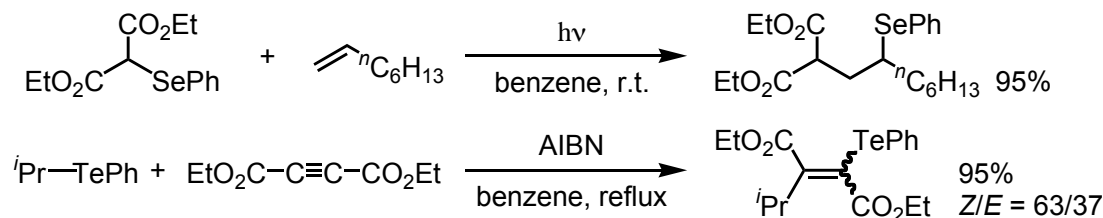
Scheme 3.11. Group-transfer reactions of organic selenium and tellurium compounds.
