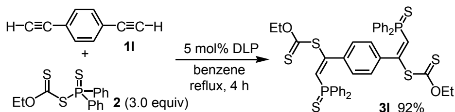
Scheme 4. Double addition of 2 to diacetylene 1l .
