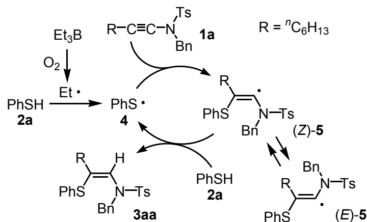
Scheme 2. Plausible reaction mechanism.
