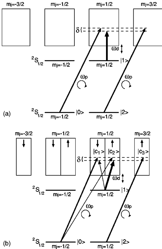
FIG. 1. Level scheme for the case in which the probe laser is right-circularly polarized, while the dressing laser is linearly polarized. (a) Naive (and misleading) picture. (b) Correct picture for which detailed results are presented in this paper. Line thickness in (b) indicates coupling strength.
