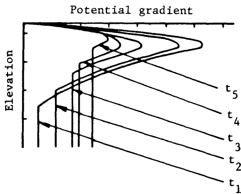
Fig.4.8 Instantaneous potential profiles
