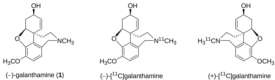
Fig. 1. Chemical structures of (-)-galanthamine, (-)- and (+)-[ ^{11}\text{C} ]galanthamine.
