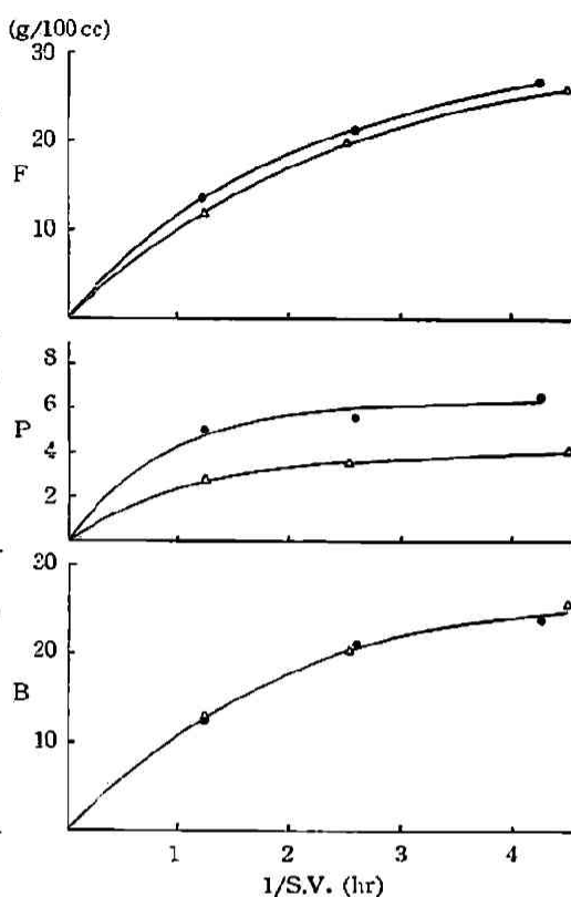
Fig. 4 Pressure effect
