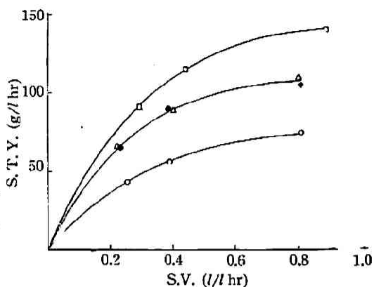
Fig. 6 Relations between S.T.Y. of butynediol and S.V.
