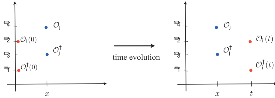
Fig. 1. The orbit of the chiral part of operators in the complex plane.
