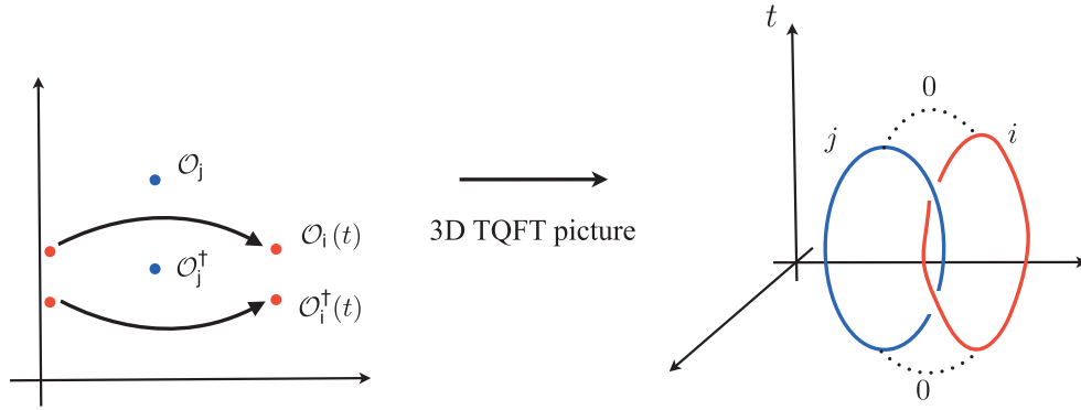
Fig. 2. 3D TQFT counterpart. Here, 0 denotes the identity channel of the conformal blocks.
