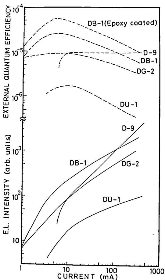
Fig. 18 Electroluminescence intensity and external quantum efficiency vs. current intensity for an undoped diode(DU-1), an Al-doped diode(D-9), a Ga-doped diode(DG-2), and a B-doped diode(DB-1). For DB-1 the characteristics after epoxy coating are also shown.
