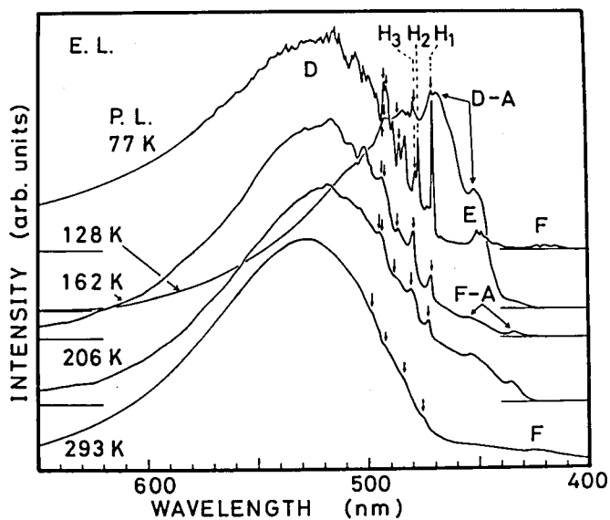
Fig. 17 Electroluminescence spectra at various temperatures and PL spectrum at 77 K of D peaks.
