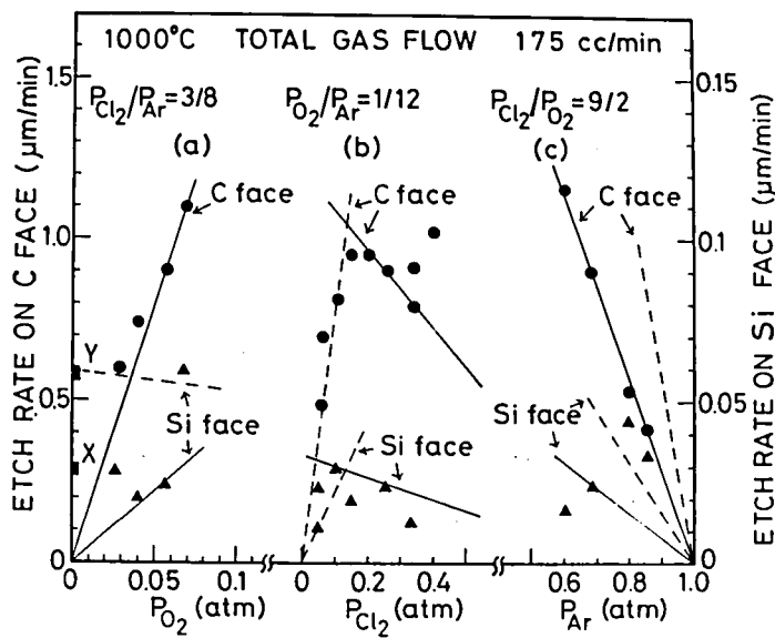
Fig. 5 Etch rate under various gas compositions at 1000^\circ\text{C} . The circles are for C faces and triangles for Si faces. The square denoted by X indicates the etch rate with a carbon film and that denoted by Y indicates that after removing the carbon film. Solid lines denote the calculated lines of L_{\text{O}_2} and broken lines of L_{\text{Cl}_2} from Eq. (13). The L_{\text{O}_2} line in the case of constant P_{\text{Cl}_2}/P_{\text{Ar}} is out of range of Fig. 5(a).
