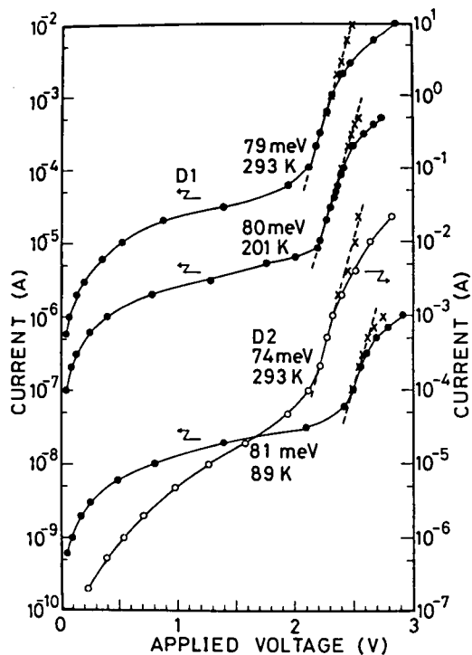
Fig. 2 Current vs. voltage characteristics of D1 and D2 at various temperatures. The crosses indicate the data after subtracting the voltage drops due to series resistances.
