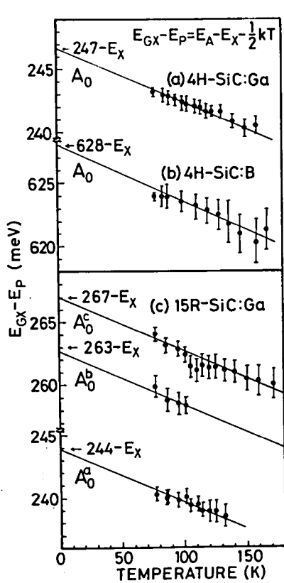
Fig. 4 Temperature dependences of E_{GX} - E_P = E_A - E_X - kT/2 for A peaks of (a) Ga-doped 4H SiC, (b) B-doped 4H SiC, (c) Ga-doped 15R SiC, (d) Al-doped 6H SiC, and (e) Ga-doped 6H SiC. The vertical bars indicate possible energy range of broad peaks.
