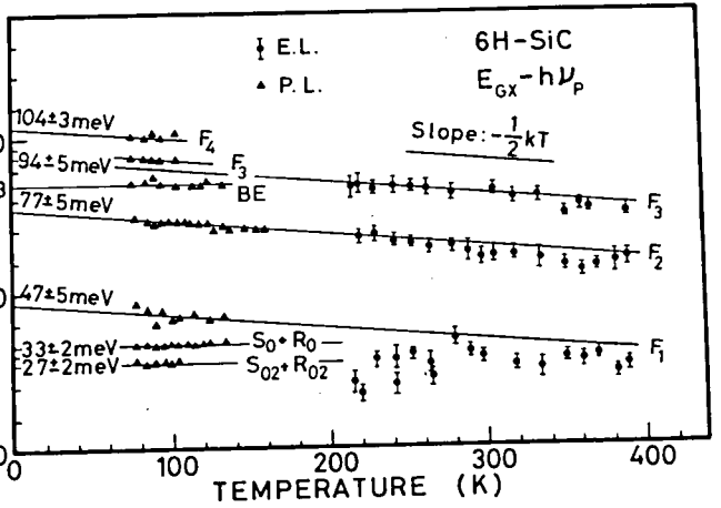
Fig. 11 Temperature dependence of E_{GX} - h\nu_p for F peaks of 6H SiC.
