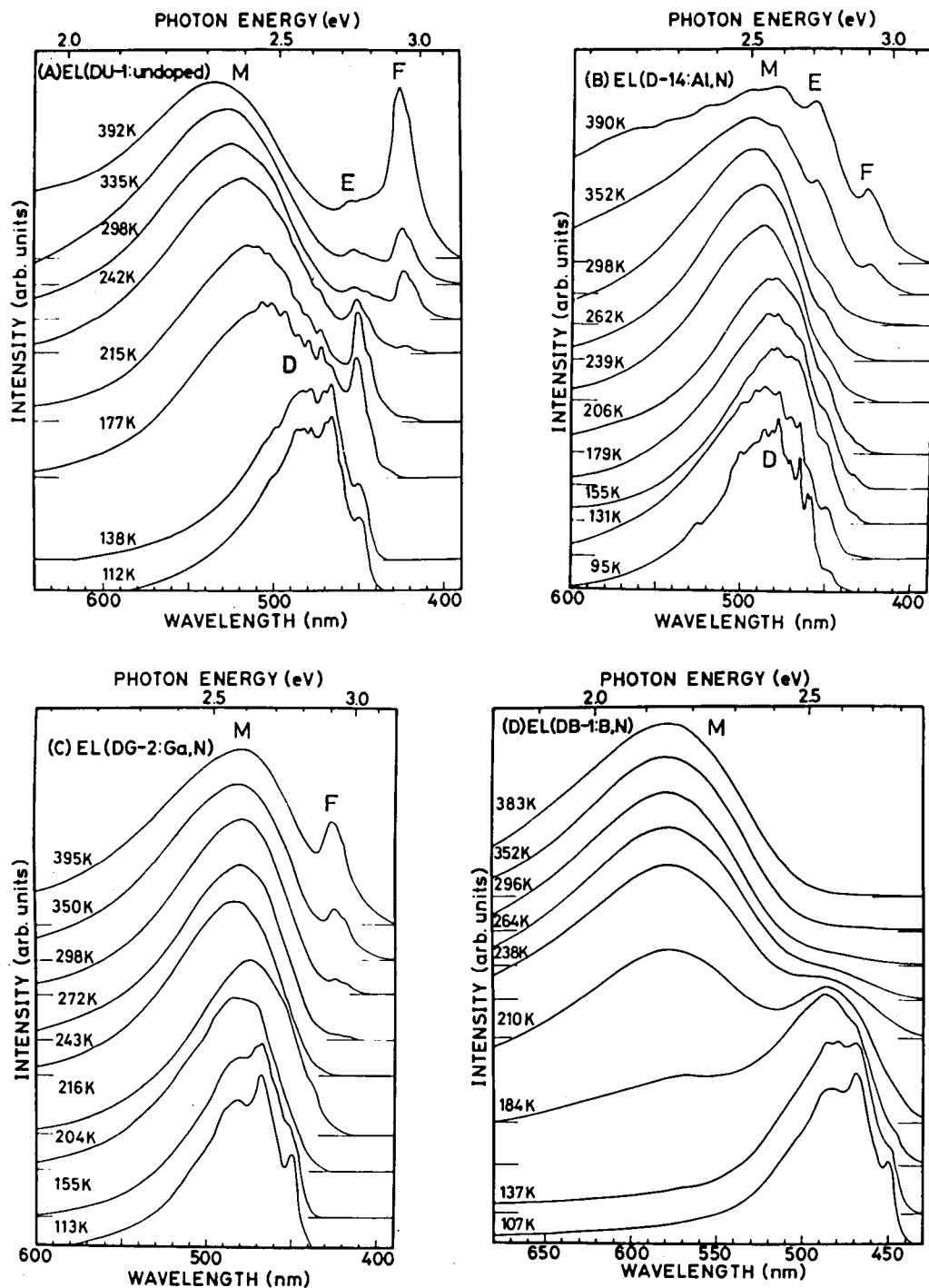
Fig. 4 Temperature dependence of the EL spectra for (a) an undoped diode, (b) an Al-doped diode, (c) a Ga-doped diode, and (d) a B-doped diode.
