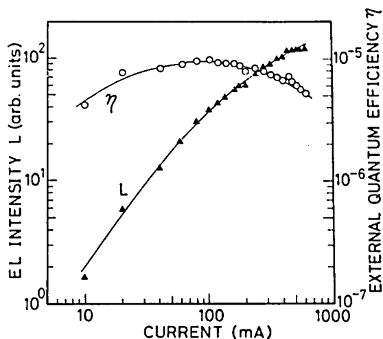
Fig. 4 Electroluminescence intensity (L) and external quantum efficiency ( \eta ) at room temperature as functions of current.
