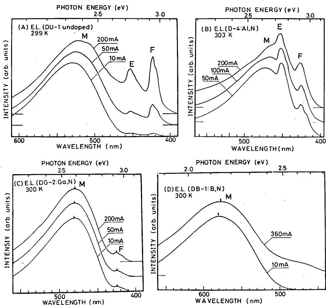
Fig. 7 Electroluminescence spectra under various driving currents for (a) an undoped diode, (b) an Al-doped diode, (c) a Ga-doped diode, and (d) a B-doped diode.
