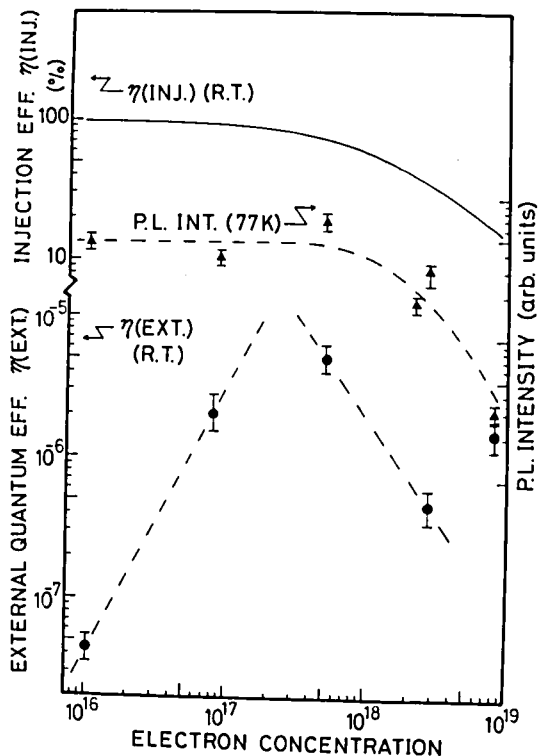
Fig. 19 Dependence of the external quantum efficiency of Al-doped diodes, the PL intensity of the n layers at 77 K, and the injection efficiency on the electron concentration of the n layers at room temperature.
