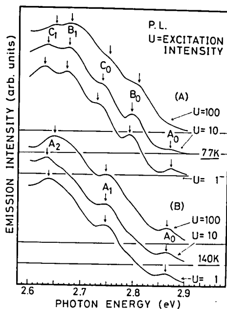
Fig. 6 Photoluminescence spectra of 6H SiC:Al,N under various excitaion intensities at (a) 77 K and (b) at 140 K.
