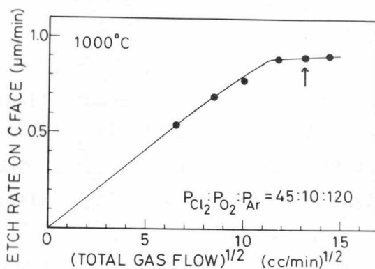
Fig. 3 Etch rate vs. square root of total flow at 1000^{\circ}\text{C} for C faces.
