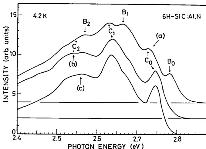
Fig. 9 Photoluminescence spectra of 6H SiC with various concentrations of Al and N impurities. (a) n = 4 \times 10^{17} \text{ cm}^{-3} (grown from Si melt with 0.01 at. % Al), (b) n = 2 \times 10^{19} \text{ cm}^{-3} (2.5 at. % Al) and degenerated, and (c) p = 2 \times 10^{18} \text{ cm}^{-3} (2.5 at. % Al).
