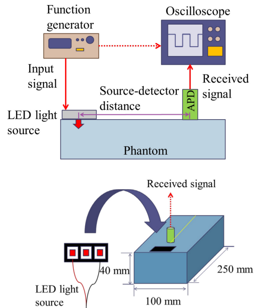
Fig. 1: Experimental setup for pulse shape analysis.
