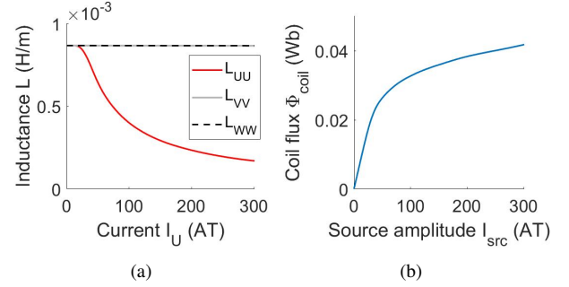
Fig. 4. (a) Self-inductances L_{UU} , L_{VV} , and L_{WW} with q = 1 . (b) Magnetic flux interlinking the coils.
