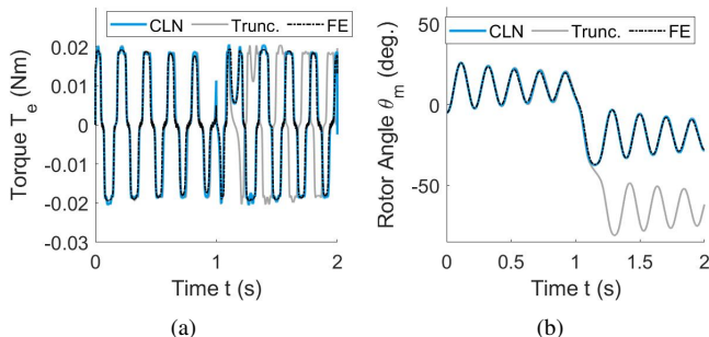
Fig. 7. Time evolution of the (a) torque and (b) rotor angle when the load torque is small. A step-out motion is observed at t = 1 s.
