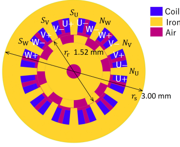
Fig. 2. Configuration of the VR stepper motor model analyzed in this study.
