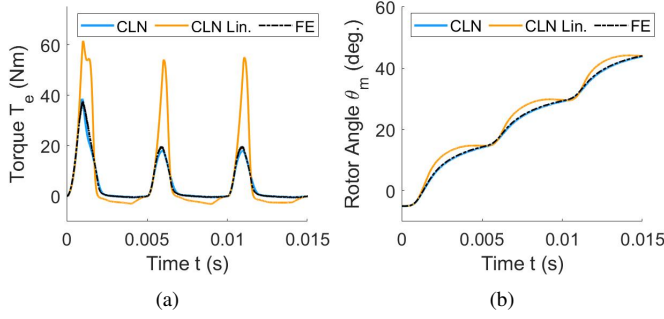
Fig. 5. Time evolution of (a) electromagnetic torque and (b) rotor angle calculated using the parameterized CLN method (CLN), linear CLN (CLN Lin.), and FE analysis (FE).
