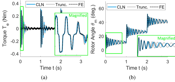
Fig. 6. (a) Torque and (b) rotor angle of stepwise rotation. The results of the truncated network (Trunc.) are also shown.
