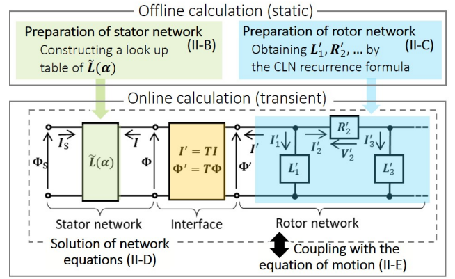
Fig. 1. Overview of the motor analysis using the parameterized CLN method.
