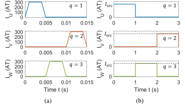
Fig. 3. (a) Trapezoidal and (b) rectangular current inputs.
