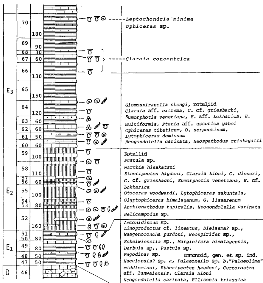
Fig. 8. Columnar section of Member E of the Khunamuh Formation.
