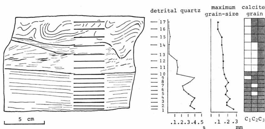
Fig. 14. Sketch of weathered surface of a limestone layer of Bed 65 showing the position of horizontal thin-sections (left), and results of thin-section analyses (right). (See also Pl. 10, Fig. 6)
