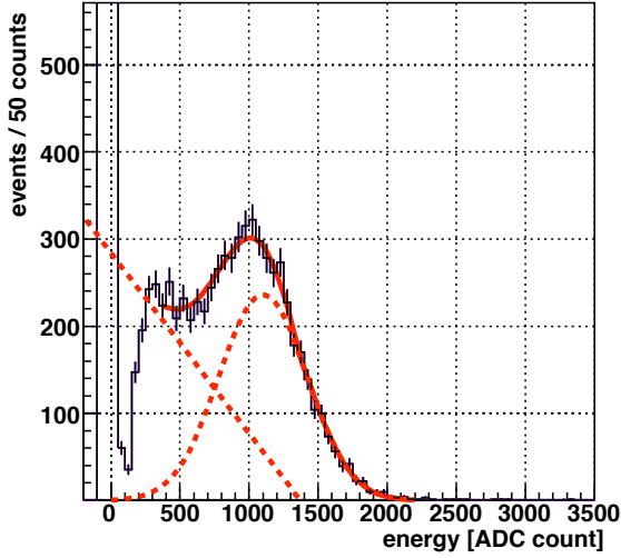
Figure 4.4: ^{137}\text{Cs} peak of the ADC distribution. The least squares fit result is shown in red solid line. The fit function consists of the photo-electron peak and the Compton edge shown in red dashed lines.
