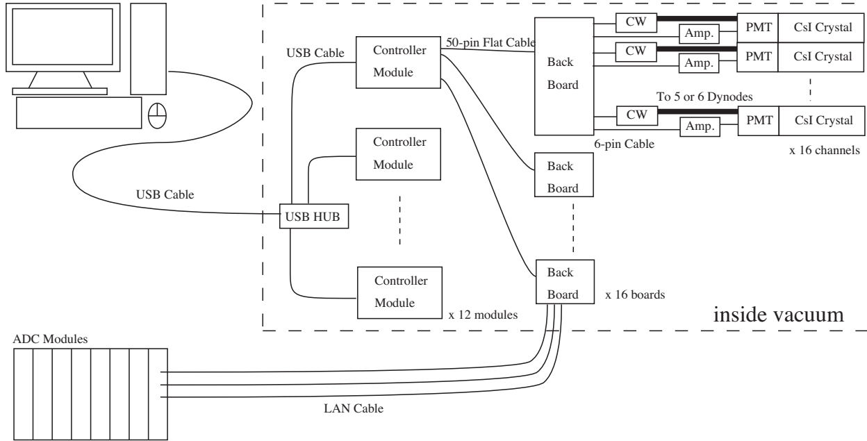
Figure 2.21: Overview of the HV control system. For the analog signals sent by the Back Boards to the ADC modules, we made the unconventional choice of using LAN cables.
