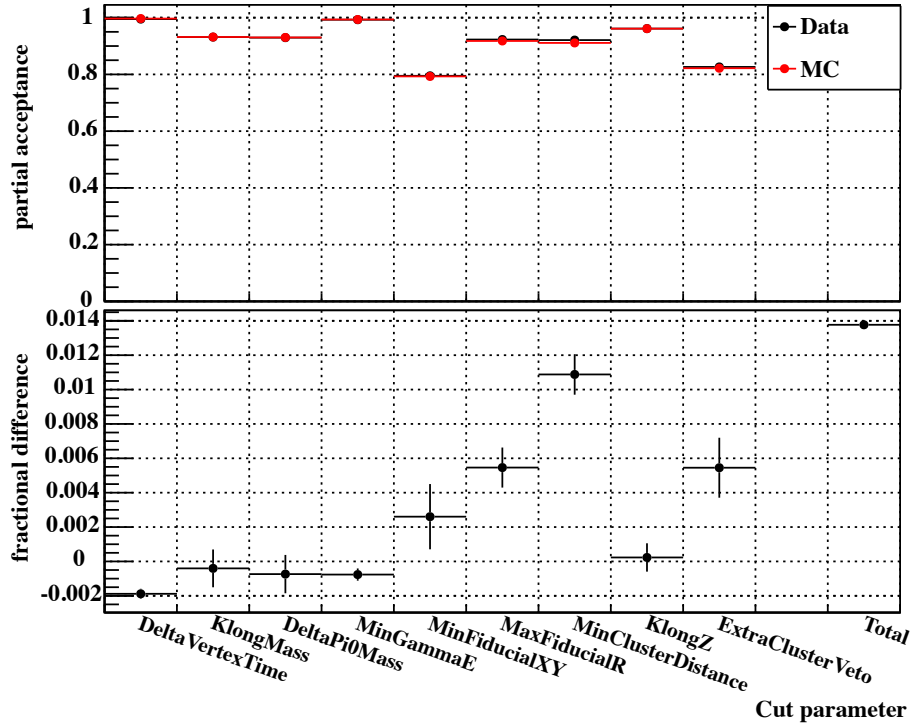
Figure 5.44: Partial acceptance (top) and Cut effectiveness (bottom) of K_L \rightarrow 3\pi^0 .
