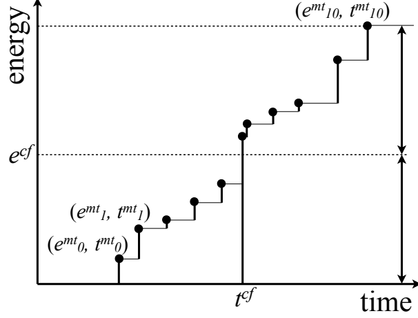
Figure 4.3: Cartoon of the pseudo pulse shape simulation. The eleven black dots represent the mtime array for one module. The horizontal axis, time, shows the each hit time of mtime, and the vertical axis, energy, shows the integrated energy until the specified time. t^{cf} is determined when the integrated energy exceed the e^{cf} .
