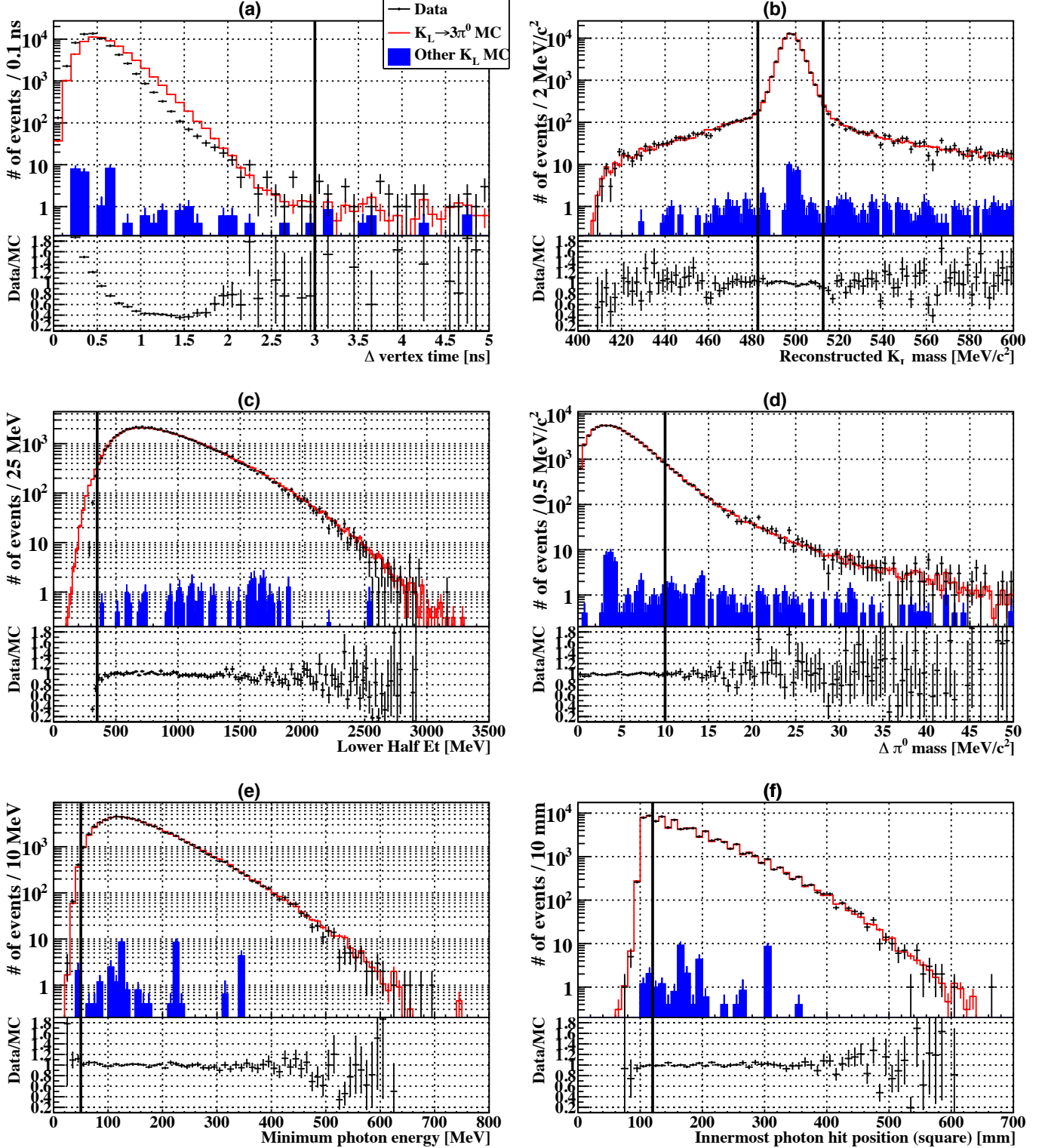
Figure 5.35: The parameter distributions of each selection for the K_L \rightarrow 3\pi^0 mode. (a) \Delta vertex time, (b) Reconstructed K_L mass, (c) Lower Half Et, (d) \Delta \pi^0 mass, (e) Minimum photon energy, (f) Hit position (square) of the innermost photon. In each figure, the black solid points represent the experimental data, the red hollow histogram is the K_L \rightarrow 3\pi^0 MC simulation, and the histogram shown in solid blue is the other K_L MC simulation. All MC distributions are normalized by the result of the K_L flux measurement. The histograms of MC simulations are stacked in order. The lower graph of each distribution shows the ratio between the experimental data and the MC simulation. Solid vertical bars in each distribution represent the threshold of each selection.
