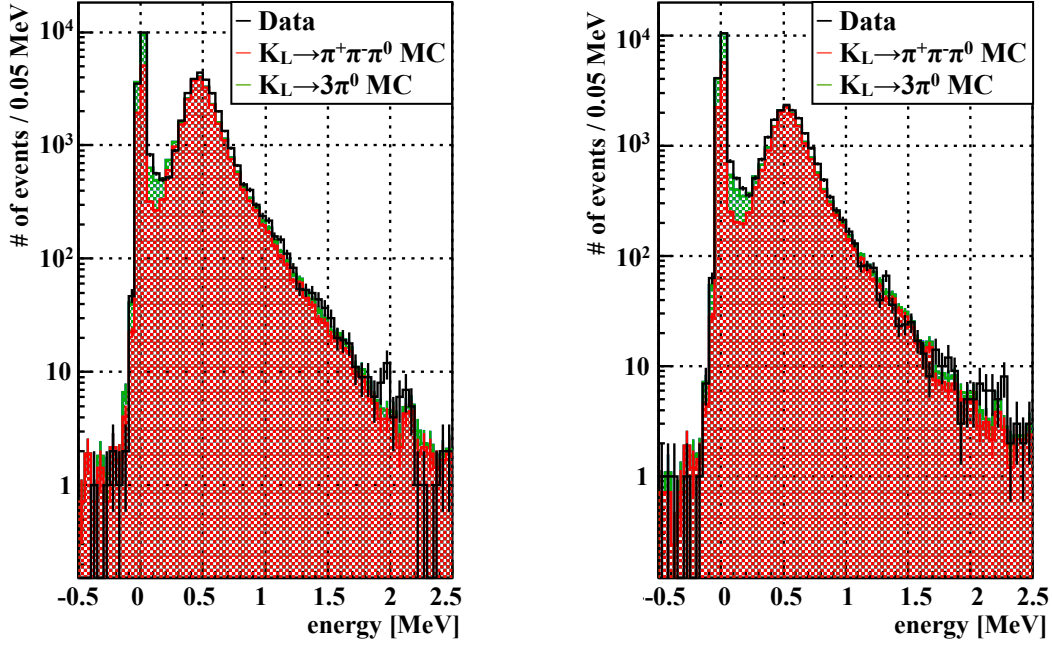
Figure A.7: Two examples of energy distributions of CV modules with the K_L \rightarrow \pi^+\pi^-\pi^0 enhancement. The innermost module (left) and the adjacent module (right) are shown. The horizontal axes are the energy deposit of each module. The black histograms show the experimental data, the red hatched histograms show the K_L \rightarrow \pi^+\pi^-\pi^0 MC result, and the green hatched histograms show the K_L \rightarrow 3\pi^0 MC result. The green hatched histograms are stacked on the red hatched histograms. The MC simulation results were normalized by the number of K_L .
