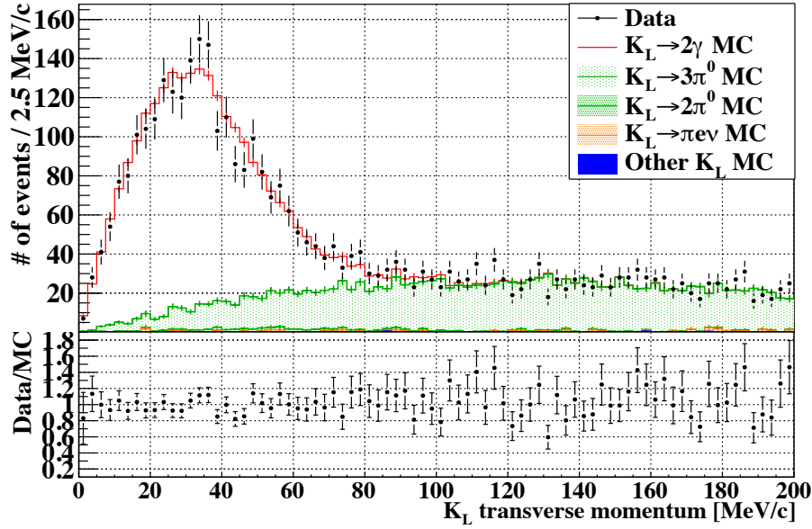
Figure 5.32: Reconstructed K_L transverse momentum spectrum with the K_L \rightarrow 2\gamma selection. The black dots show the experimental data, the red hollow histogram shows K_L \rightarrow 2\gamma MC simulation, the green light hatched histogram shows K_L \rightarrow 3\pi^0 MC simulation, the green dark hatched histogram shows K_L \rightarrow 2\pi^0 MC simulation, orange hatched histogram shows Ke3 MC simulation, and the blue histogram shows the other MC simulations. The MC histograms are normalized by the K_L \rightarrow 3\pi^0 result, and they are stacked in order.
