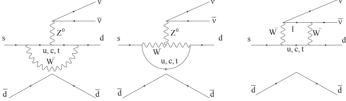
Figure 1.1: Feynman diagrams for K_L \rightarrow \pi^0 \nu \bar{\nu} .
