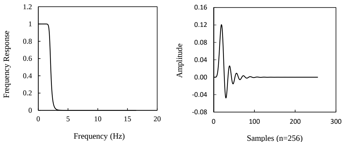
(a). Frequency response of digital low pass filter
