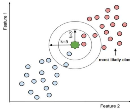
Figure 2-16 KNN classification for a two-class problem when the K parameter is set to “3” and “5”. The green star represents a unseen sample point [55].
