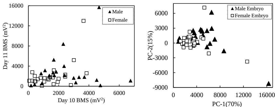
(a) Scatter plot of male and female embryos' BMS at days 10-11
