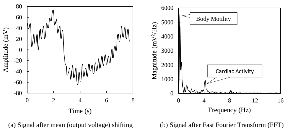
Figure 5-4 Typical signal (a) and corresponding FFT signal (b) of an embryo at incubation day 15. The small, rapid waves (high-frequency component) in (a) represent heart beats and big, slow changes (low-frequency component) represent body movement.
