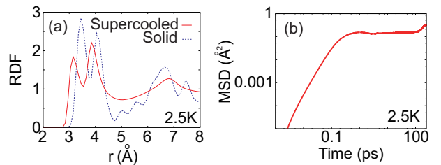
Fig. 1 (a) Comparison of RDFs of the supercooled liquid and solid at 2.5 K. The RDF of the supercooled liquid did not have a long-range periodic structure and its first peak appeared at the shorter distance in spite of the lower overall density. (b) MSD of the supercooled liquid at 2.5 K. The MSD showed plateau and collapse stages and was not on a linear line.
