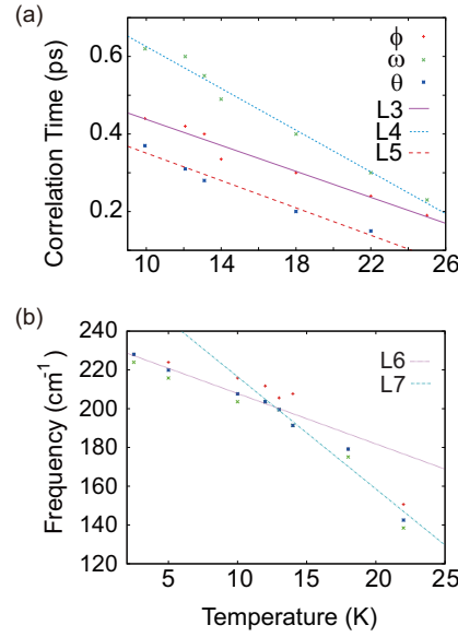
Figure S9: (a) Short correlation times of the self-orientations \phi and \omega and the intermolecular angle \theta as a function of temperature. The short correlation times simply reflect kinetic dynamics inside a cluster and were on the single linear line: L3=16.75x + 605.2 , L4=-26.93x + 894.7 , and L5=-17.65x + 527.2 . We note that the decay of the correlation function at below 10 K was reproduced only by the single Gaussian function not by the multiple exponential functions. This is because the translational motions such as cluster deformations were almost suppressed at below 10 K, and the correlations were decayed by the simple orientational motions inside a lattice cluster.
