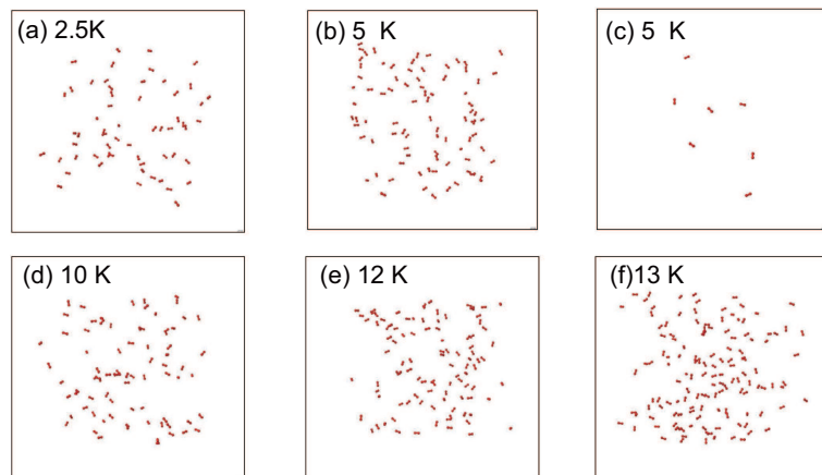
Figure S3: Snap shots of \text{H}_2 molecules which have kinetic energy larger than (a) 3.00 K, (b) 5.89 K, and (c-f) 12.0 K. As seen in (a), (b) and (d-f), \text{H}_2 molecules of high kinetic energy did not exist randomly but rather irregularly in the simulation box, which is a typical property of supercooled liquid. The panel (c) demonstrates that there were only a few \text{H}_2 molecules having kinetic energy higher than 12.0 K and significant translational motions were almost frozen at the temperature of 5 K. This fact rationalizes the disappearance of the translational peak at the extremely lower temperature in Fig.2.
