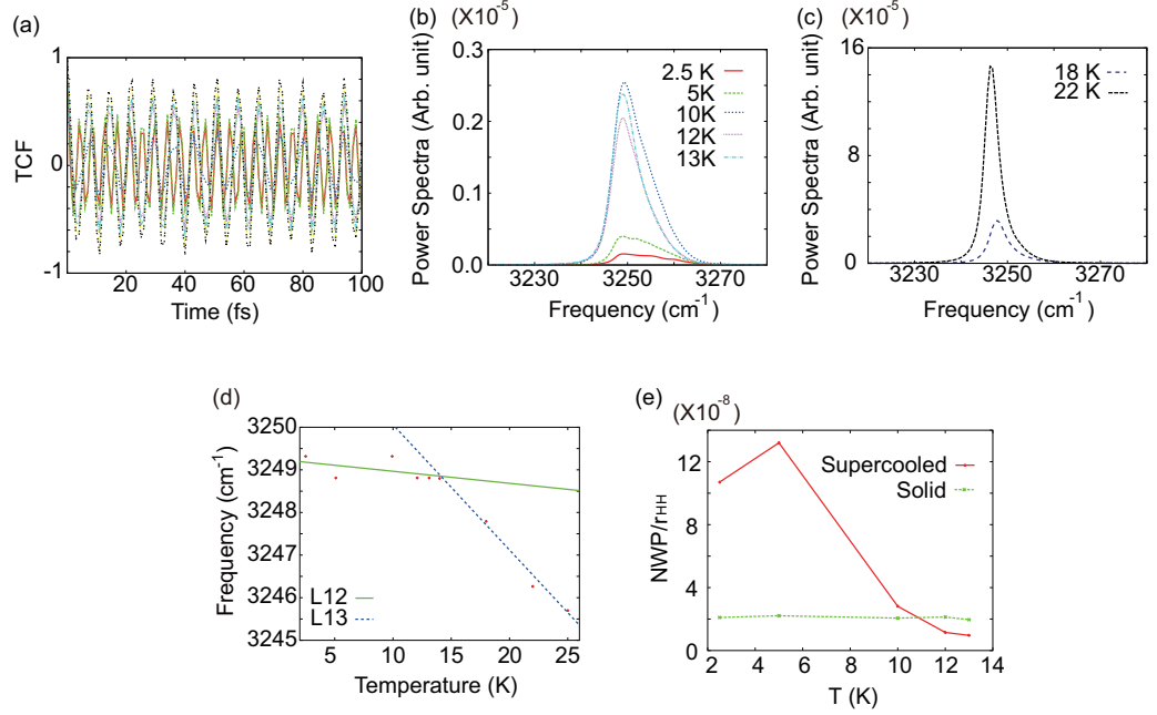
Figure S11: (a) Time correlation functions of the NWP width as a function of time. The amplitude is linked to the variations of the NWP width-distributions in Fig.4(a).
