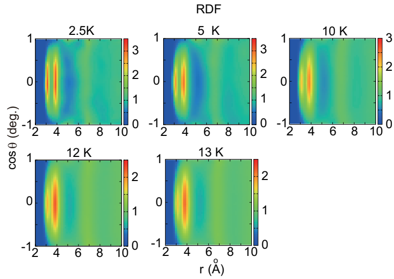
Figure S2: 2D RDFs as a function of a radial coordinate r and the intermolecular angle \theta . [2] No long-range periodic structure was obtained unlike the 2D RDFs of the \text{H}_2 solid. The whole shapes were rather close to the 2D RDFs of the normal liquid. [2, 3]
