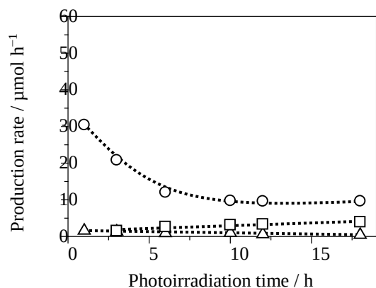
Fig. 4. Time courses of the production rates of \text{CO} (circle), \text{H}_2 (triangle), and \text{O}_2 (square) in the photocatalytic reduction of \text{CO}_2 with water over the \text{Ag}(3.5)/\text{CaTiO}_3 sample without the \text{CO}_2 bubbling flow.
