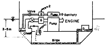
Fig. 5. The method of measuring the water temperature in Ferry Boat. Thermistor sensor is attached in the sanitary strainer (S).
