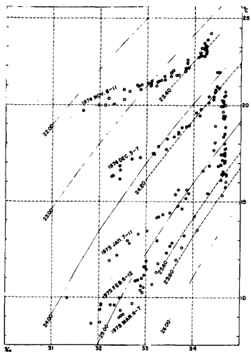
Fig. 4. T-S diagram at Kii Channel in winter.
