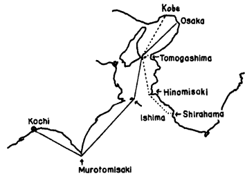
Fig. 6. Course of Ferry "Katsura" (solid line) and Ferry "Katsuura" (dotted line)
