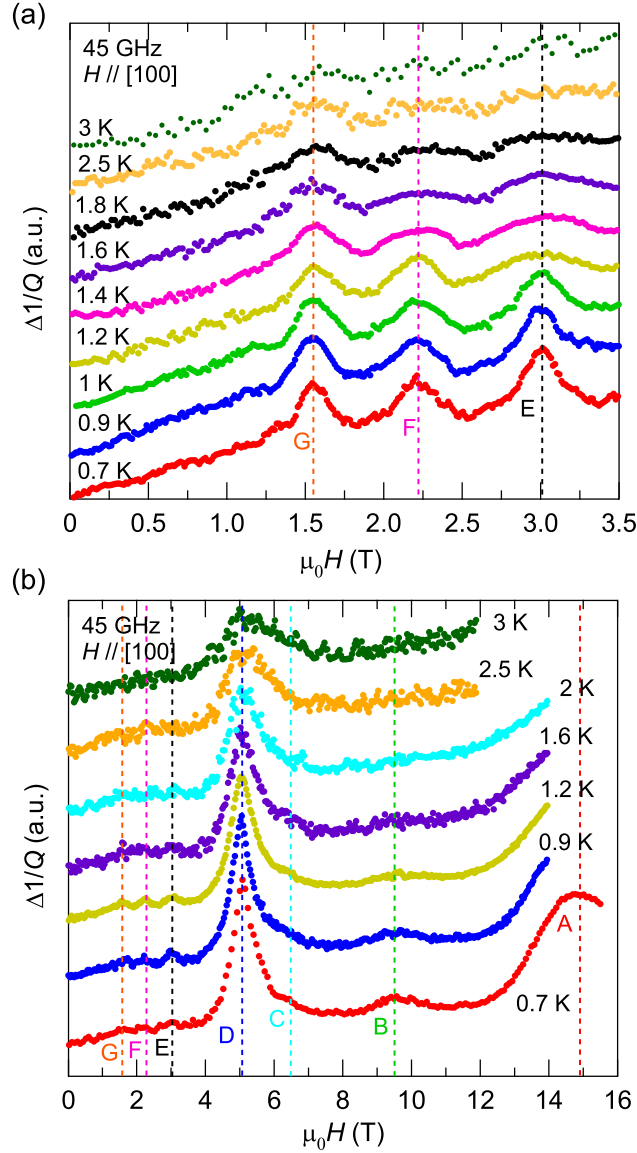
Figure 5.4: Observation of cyclotron resonance in the superconducting phase of \text{URu}_2\text{Si}_2 . (a) Field dependence of the change 1/Q at several temperatures for \mathbf{H} \parallel [100] .
