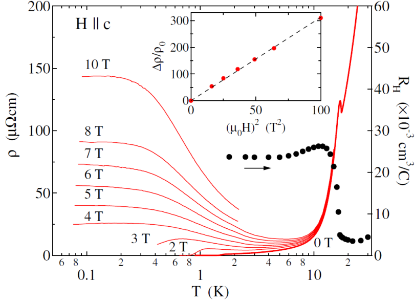
Figure 2.5: The temperature dependence of resistivity \rho (solid lines) in zero and finite magnetic fields ( \mathbf{H} \parallel c ) and the Hall coefficient R_H (solid circles). Inset shows the magnetoresistance at T \rightarrow 0 K as a function of H^2 [29].
