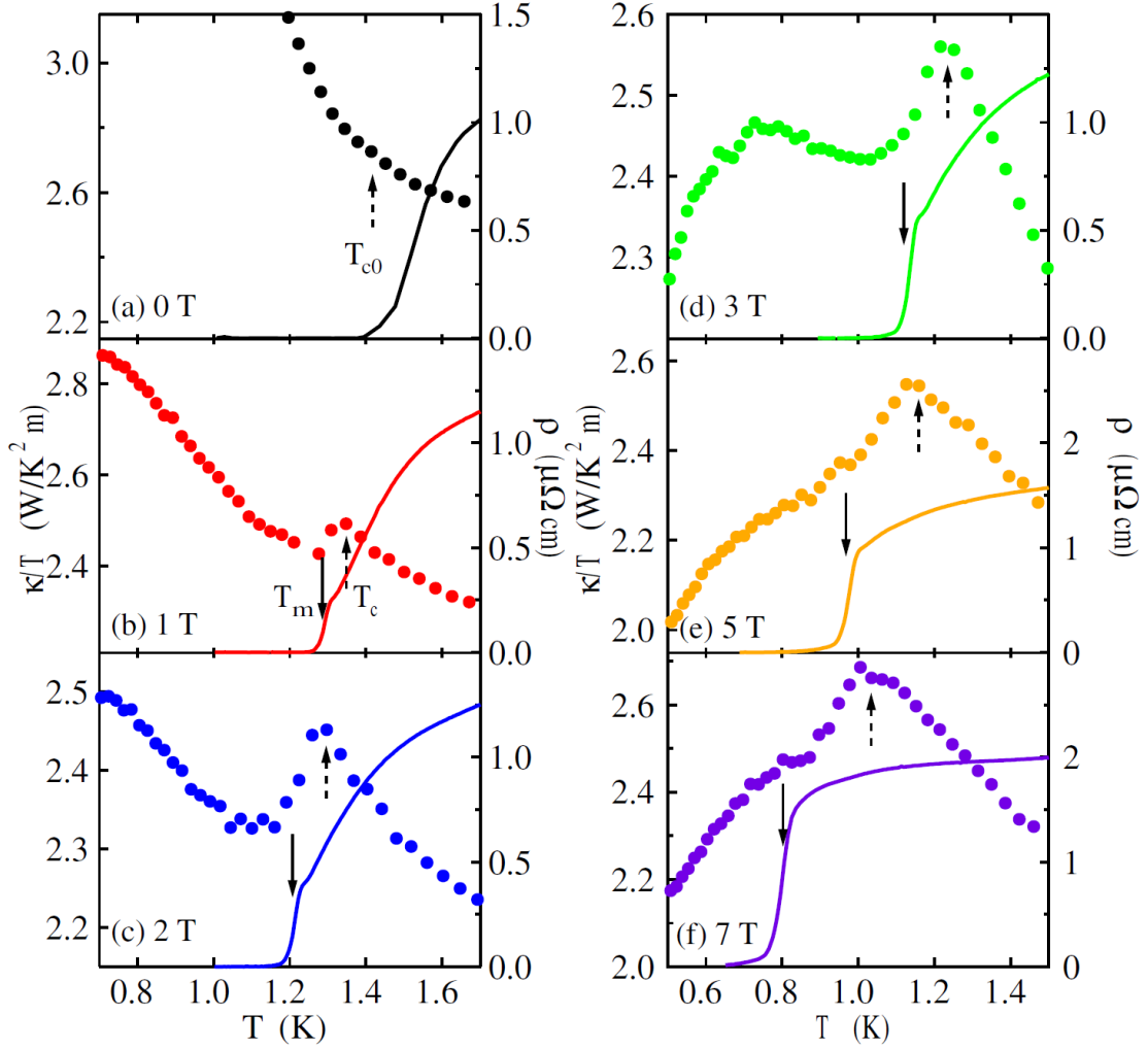
Figure 2.21: Temperature dependence of \kappa/T (left axis) and \rho (right axis) measured in several magnetic fields for H \parallel a . The dotted arrow indicates a cusp at T_{\text{SC}}(H) . The solid arrows denote the melting temperature T_m [73].
