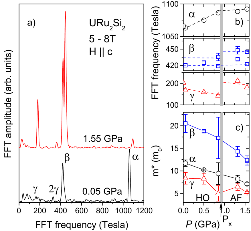
Figure 2.10: (a) FFT spectra of SdH measurements in \text{URu}_2\text{Si}_2 for H \parallel c at the lowest temperature of T \simeq 35 mK for P = 0.05 GPa and T \simeq 35 mK for P = 1.55 GPa. (b) Pressure dependence of the FFT frequencies. (c) Pressure dependence of the effective masses determined in a field range of 8-13 T [34].
