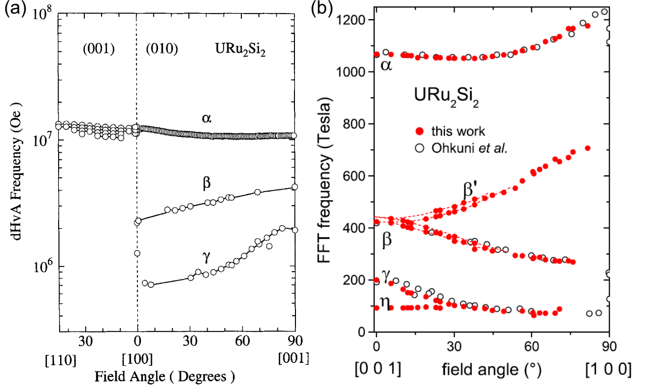
Figure 2.9: Field angular dependence of the FFT frequencies obtained from (a) dHvA [33] and (b) SdH [34] measurements in \text{URu}_2\text{Si}_2 , reflecting the cross sectional areas of the different Fermi surface branches perpendicular to the magnetic field. The dHvA results are also plotted in (b) SdH results and are in excellent agreement.
