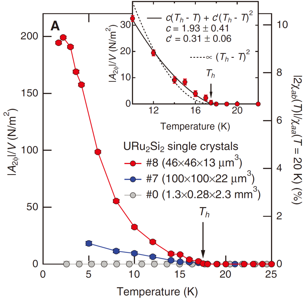
Figure 2.14: Temperature dependence of two-fold oscillation amplitude divided by the sample volume |A_{2\phi}|/V . The normalized in-plane susceptibility anisotropy |2\chi_{ab}(T)|/\chi_{aa}(T = 20 \text{ K}) = (C - \chi[1\bar{1}0])/\chi[100] is evaluated in the right axis [27].
