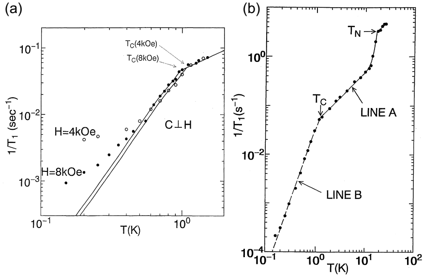
Figure 2.17: (a) Temperature dependence of 1/T_1 of 29 Si obtained by 29 Si NMR [68]. (b) Temperature dependence of 1/T_1 of 101 Ru obtained by 101 Ru NMR [69].
