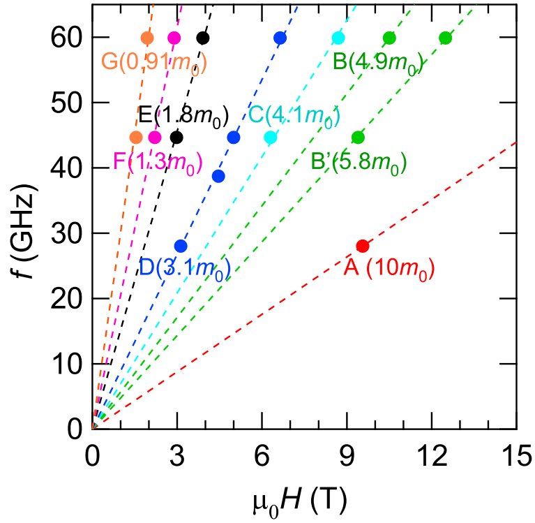
Figure 4.10: Relation between the measured frequencies and the resonance fields for \mathbf{H} \parallel [100] .
