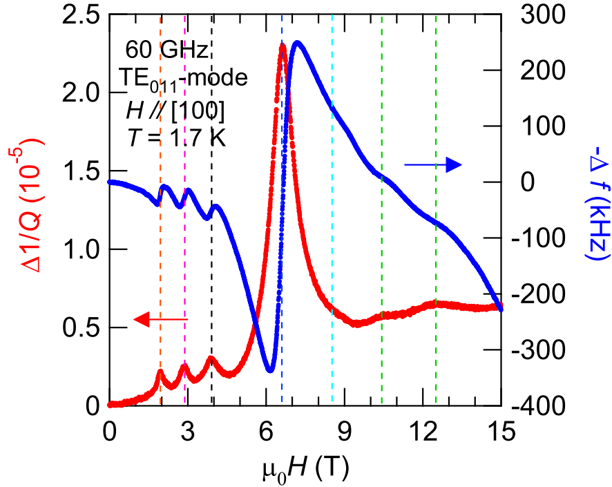
Figure 4.8: Magnetic-field dependence of the change in the microwave dissipation \Delta 1/Q (red, left axis) and the frequency shift \Delta f (blue, right axis) of the 60-GHz cavity resonator containing a single crystal at 1.7 K. The dc field is along the [100] direction. The weak field dependence measured without the crystal has been subtracted. The dotted lines mark the resonance fields.
