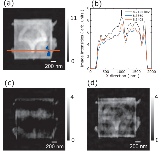
FIG. 3. (Color) (a) Image reconstructed from the diffraction pattern shown in Fig. 2(a). The pixel size is 17.4 nm. (b) One-dimensional plots of the reconstructions at 8.2125, 8.3360, and 8.3405 keV along the solid red line indicated in (a). Images are normalized by the sum of each reconstructed intensity at the blue regions in (a). Difference images for (c) 8.3360 and 8.3405 keV and (d) 8.2125 and 8.3360 keV.
