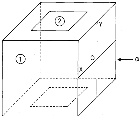
Fig. 1. Crystal surfaces coupled to two photodiodes. CsI(Tl) crystal (1) has a dimension of 20 \times 20 \times 20 mm 3 and the photosensitive surface of photodiode (2) has an area of 10 \times 10 mm 2 . Coordinate axes are defined as shown. Alpha-particles are incident on the crystal along the z axis.
