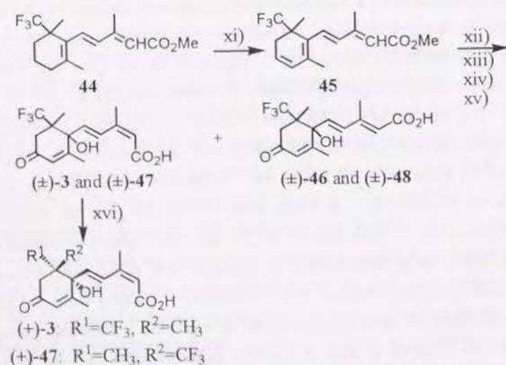
Fig. 6. Synthesis and optical resolution of 3 and 47. For xi) - xvi), see legends of Fig. 5.
