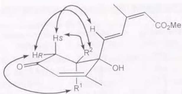
Fig. 10. Favored conformations of 1a , 4a and 62a .
