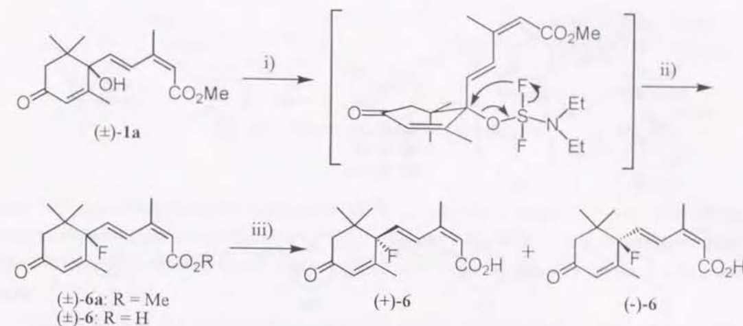
Fig. 17. Synthesis and optical resolution of 6 . i) DAST ii) esterase iii) HPLC with Chiralcel OF.
