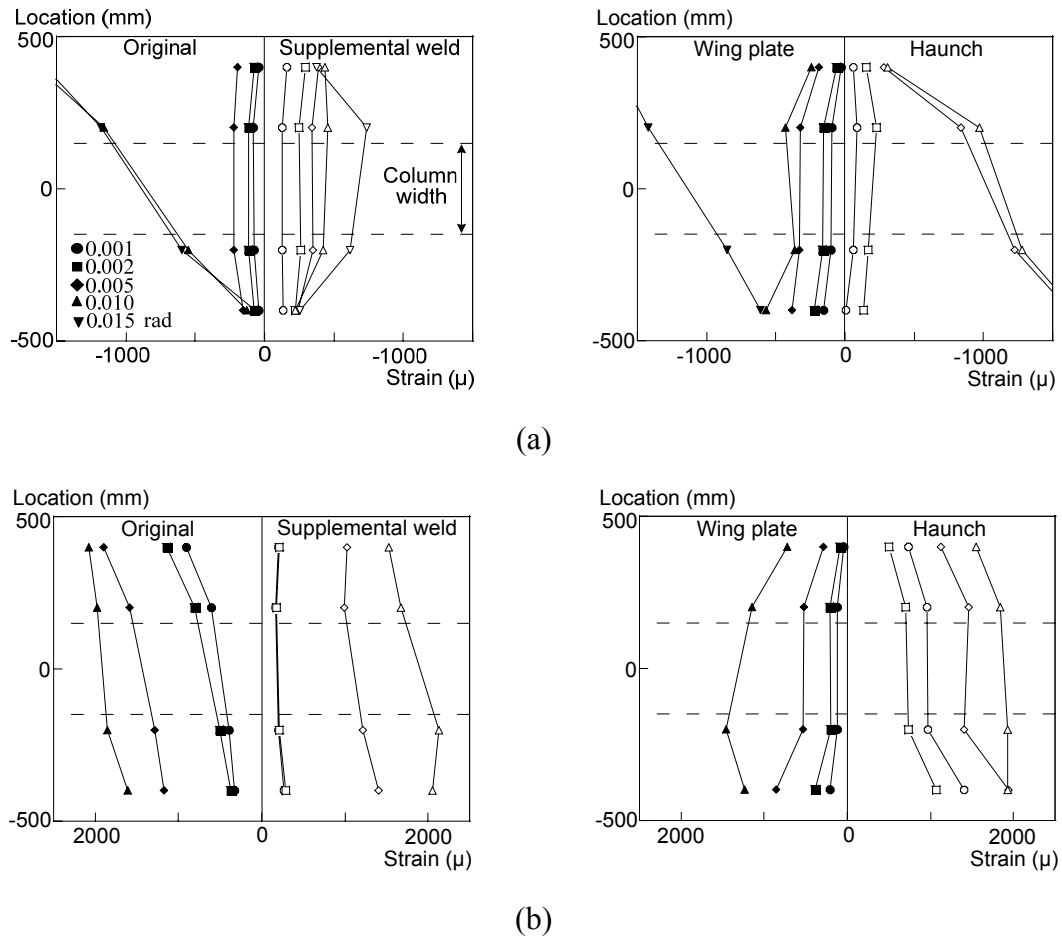
Figure 5.30 Strain distributions in steel rebars: (a) Positive bending; (b) Negative bending
