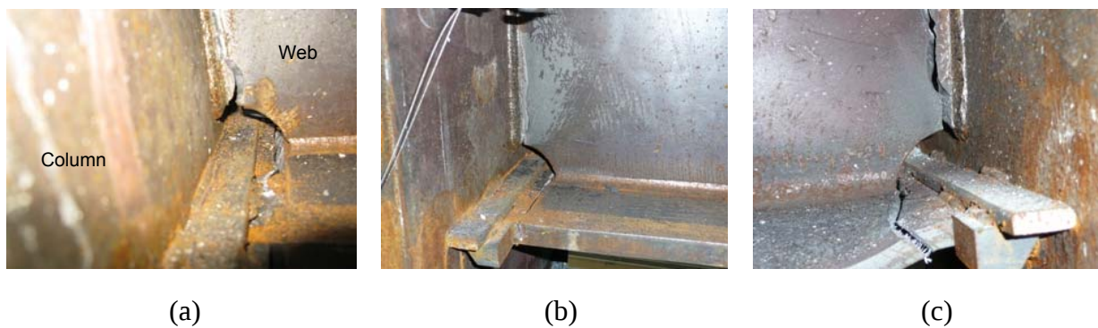
Figure 4.4 Fractures of shop weld connections: (a) Third floor (NR); (b) Forth floor (NR); (c) Third floor (SL)
