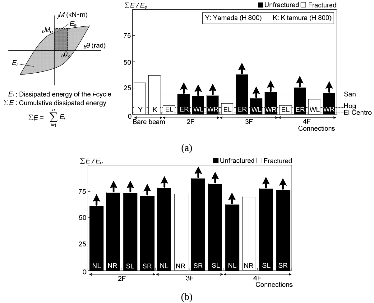
Figure 4.16 Cumulative ductility ratio of connections: (a) Field weld connections; (b) Shop weld connections
