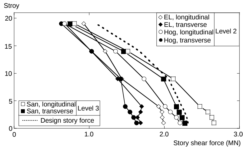
Figure 3.4 Maximum story shear force distribution
