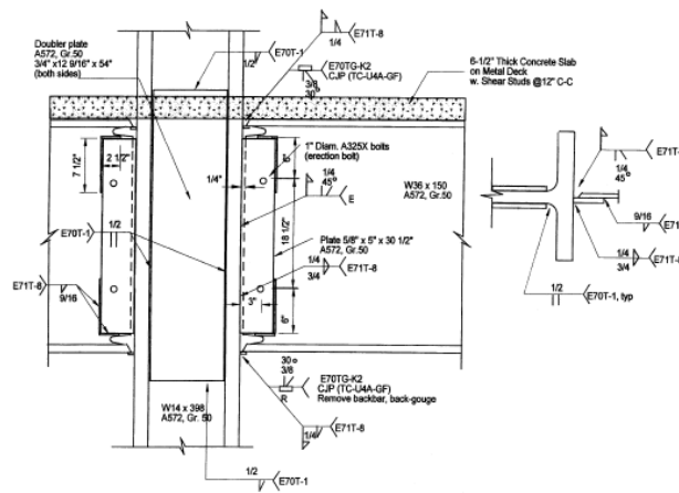
Figure 6.4 Welded unreinforced flange-welded web (WUF-W) connection (Ricles et al. 2000)
