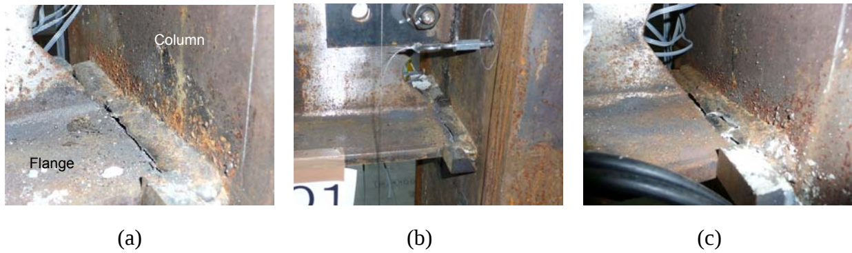
Figure 4.3 Fractures of field weld connections: (a) The second floor connection; (b) The third floor connection; (c) The forth floor connection
