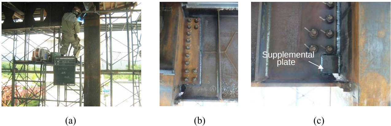
Figure 6.6 Connection with modified supplemental welds: (a) Welding situation; (b) Supplemental welds; (c) Modified supplemental welds
