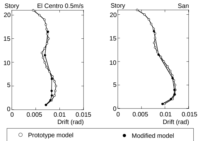
(a) (b) Figure 2.6 Inter-story drift responses of prototype model and modified model: (a) El Centro-NS 0.5m/s; (b) San-EW
