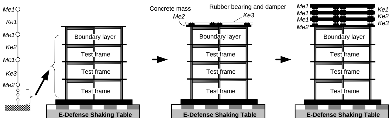
Figure 2.5 Physical image of the test specimen
