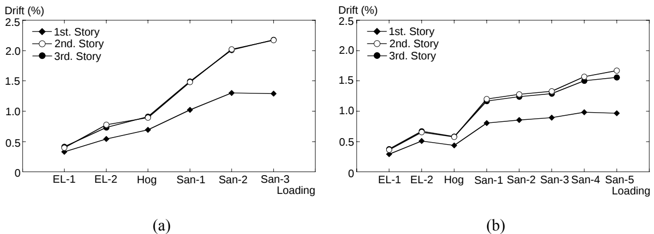
Figure 6.12 Max. inter-story drift angles: (a) Longitudinal direction; (b) Transverse direction
