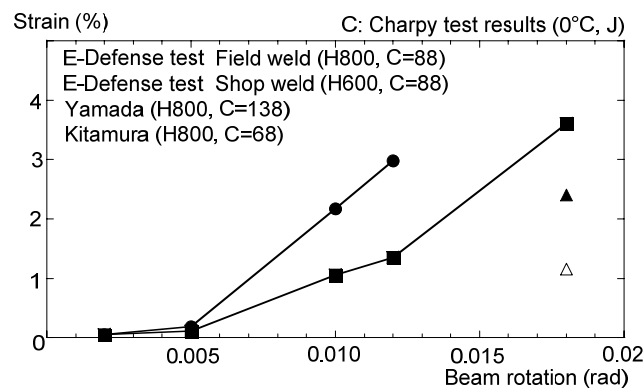
Figure 4.14 Growth of bottom flange strains
