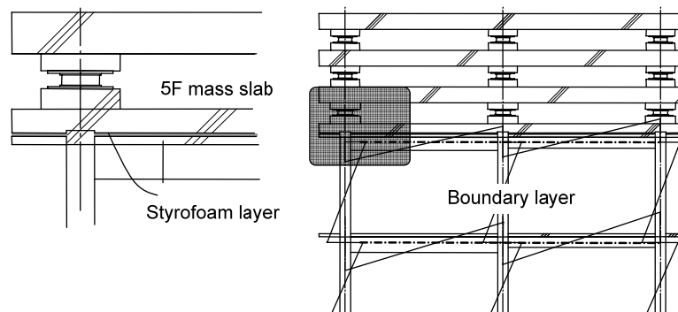
Figure 2.12 Boundary detail between the frame and substitute layers
