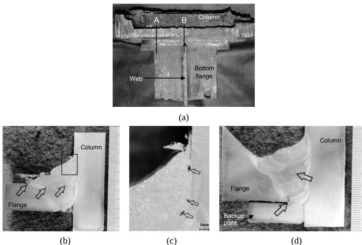
Figure 4.12 Microscopic examination of an unfractured cross-section: (a) Bottom flange specimen (the third floor, ER); (b) Section A; (c) Detail of section A; (d) Section B
