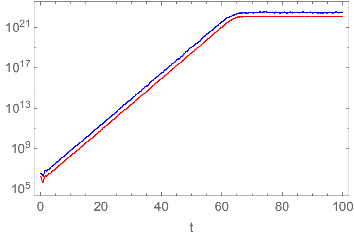
Figure 6. The correlators \langle O^{ij}(t, 0)^2 \rangle (blue) and \langle O^{jk}(t, 0)^2 \rangle (red) as a function of time, with N = 20 . t = 0 is the time of the initial perturbation.
