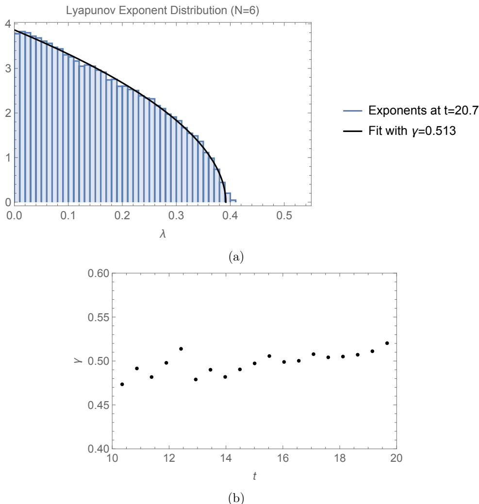
Figure 10. (a) Positive Lyapunov spectrum for N = 6 and a fit to the ansatz (5.10) at the largest t we have studied, and (b) the fitting parameters \gamma versus t . Here we normalize the area of only the positive part of the spectrum to unity, and multiply the right-hand side of (5.10) by 2 accordingly.
