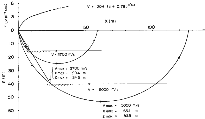
Fig. 1 A travelttime-distance curve (upper half) and ray paths (lower half) in a Mirage layer. The ray, which would reach the maximum depth z_{\max} corresponding to V_{\max} in a Mirage layer, suffers a critical-angle refraction, if it impinges on the bed rock of V = V_{\max} .
