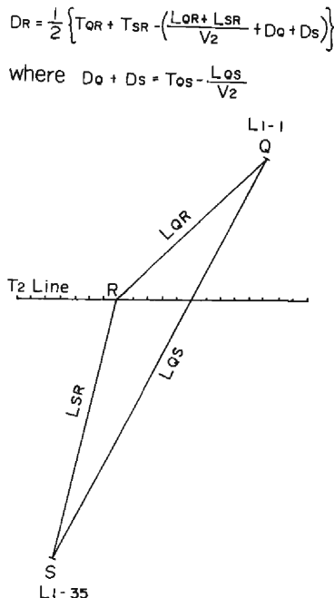
Fig. 4 The layout of measuring line T_2 for a fan shooting at Q and S . T is travel time, D_R , D_Q and D_S are the delay times at R , Q and S , respectively, and V_2 is the bed-rock velocity.
