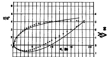
Fig. 23 Relationship among \sigma_1/\sigma_3 , \epsilon_1 and \Delta V/V (Toyoura sand).
