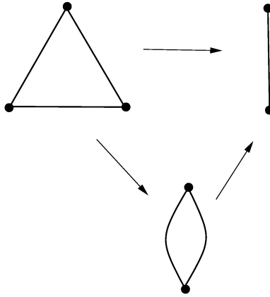
Figure 3. Stein factorization of a simplicial map
