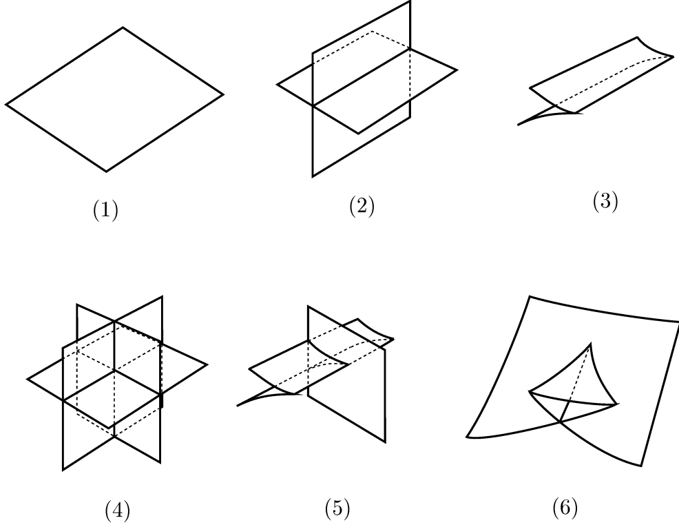
Figure 9. Multi-germs of g|_{S(g)}
