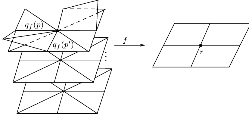
Figure 8. Multi-germ corresponding to a double cone
