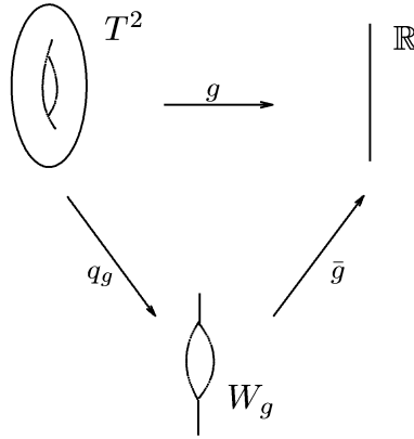
Figure 1. Stein factorization may not be a manifold
