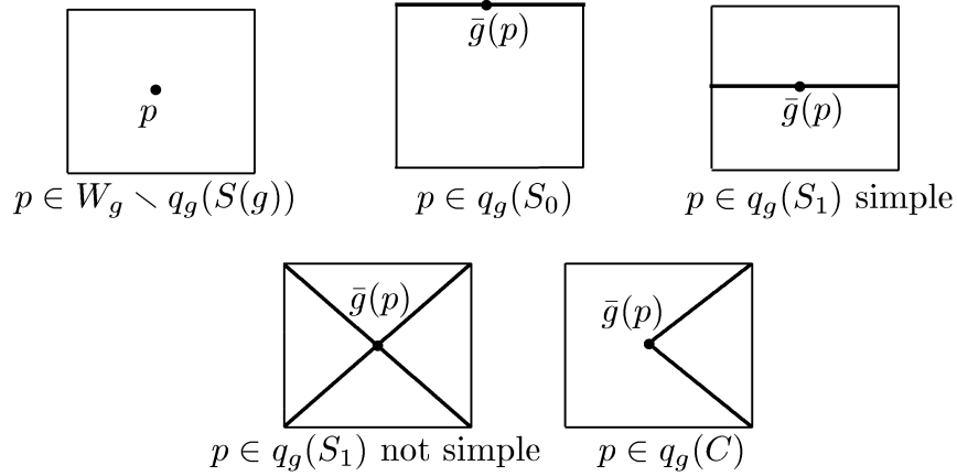
Figure 6. Images of canonical neighborhoods by \bar{g}
