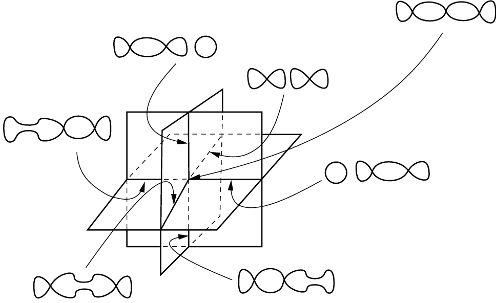
Figure 10. Degeneration of fibers near a \text{III}^4 -type singular fiber
