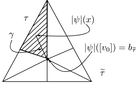
Figure 2. The simplices \tau and \tilde{\tau}
