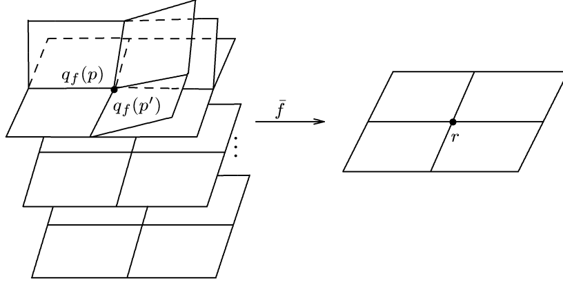
Figure 7. Multi-germ corresponding to a trident
