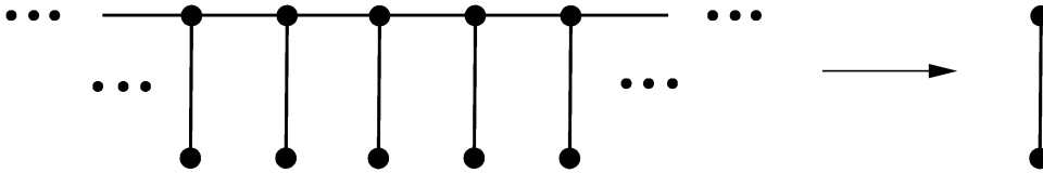
Figure 4. Example of a non-proper simplicial map
