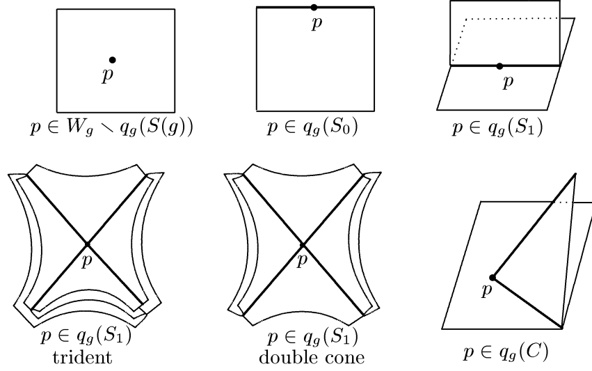
Figure 5. Local structures of W_g
