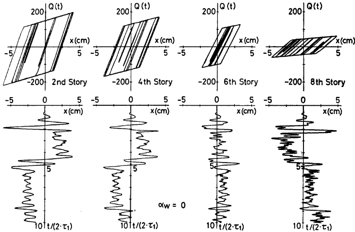
Fig. 7. Q-x and x-t relations. ( \alpha_w=0 )
