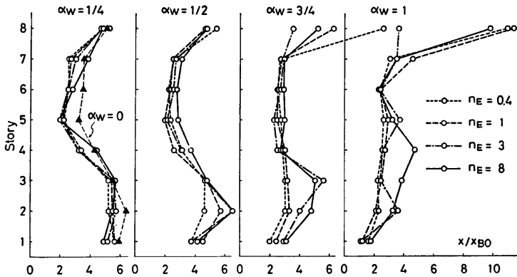
Fig. 6. Distribution of relative displacement. ( R=1.5 )
