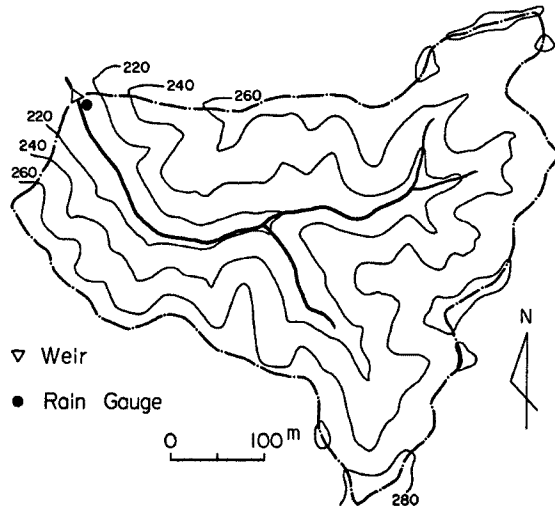
Fig. 3. Wajima-Yanagida catchment.
