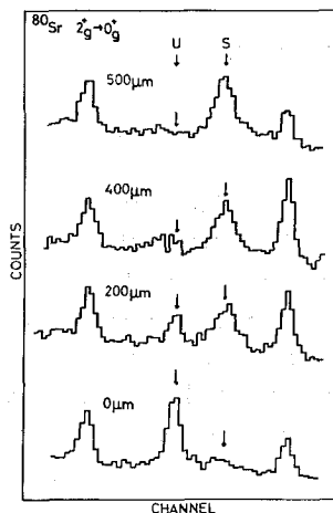
Fig. 6. A portion of the \gamma -ray spectra in the vicinity of the 385.7 keV 2^+_{\text{g}} \rightarrow 0^+_{\text{g}} transition in ^{80}\text{Sr} with various recoil distances.
