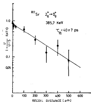
Fig. 7. The ratio I of unshifted versus sum of the shifted and unshifted peak yields for the 385.7 keV 2^+_{\text{g}} \rightarrow 0^+_{\text{g}} transition in ^{80}\text{Sr} .
