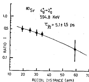
Fig. 8. The ratio I for the 594.8 keV 4^+_{\text{g}} \rightarrow 2^+_{\text{g}} transition in ^{80}\text{Sr} .
