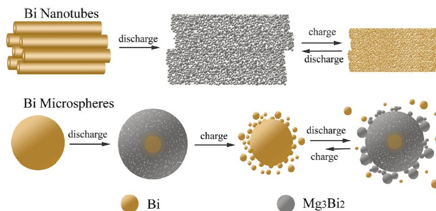
Figure 1-16. Structural transformation of bismuth during the discharge/charge process 126 .
