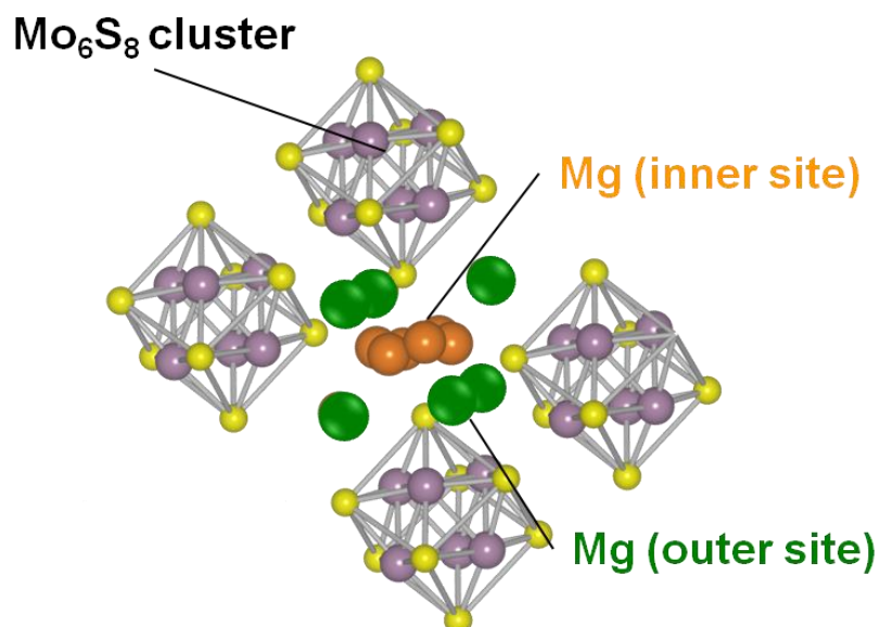
Figure 1-3. Crystal structure of the chevrel Mg 2 Mo 6 S 8 phase. Green, orange, purple, and yellow spheres are indicated Mg (outer site), Mg (inner site), Mo, and S atoms, respectively 72 .
