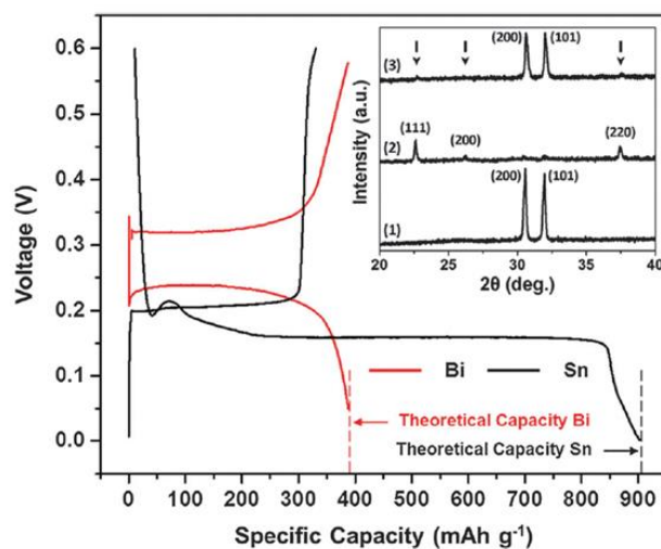
Figure 1-13. 1st cycle galvanostatic magnesiation/de-magnesiation curves for Sn/Mg (black) and Bi/Mg (red) half-cells (using organohaloaluminate electrolyte) highlighting, their achievable theoretical capacities. Inset - XRD spectra for as-fabricated Sn, (2) magnesiated Sn (or \text{Mg}_2\text{Sn} - peak positions marked with arrows) and (3) de-magnesiated \text{Mg}_2\text{Sn} 123 .
