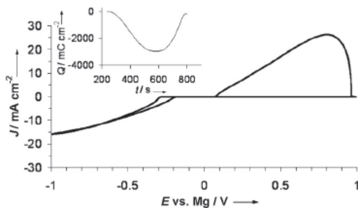
Figure 1-9. Cyclic voltammogram of \text{LiBH}_4/\text{Mg}(\text{BH}_4)_2 in glyme 113 .
