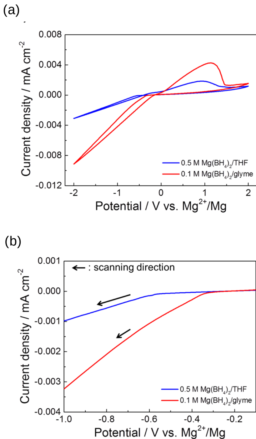
Figure 4-1. (a) Cyclic voltammograms of bismuth electrode in 0.5 M Mg(BH 4 ) 2 /THF and 0.1 M Mg(BH 4 ) 2 /glyme at a scanning rate of 20 mV/sec. (b) Enlarged figure of (a) between -1.0 V and -0.1 V (vs. Mg 2+ /Mg).
