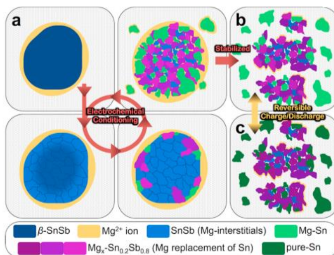
Figure 1-19. Diagram of the electrochemical \text{Mg}^{2+} insertion and extraction processes for a \beta\text{-SnSb} nanoparticle based on the TEM and DFT results 134 .
