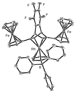
Fig. 1 ORTEP illustration of Rh((S,S)-\mathbf{1f})[(\eta^6-C_6H_5)BPh_3] with thermal ellipsoids drawn at 50% probability level. The solvent molecule ( CH_2Cl_2 ) and hydrogens are omitted for clarity.
