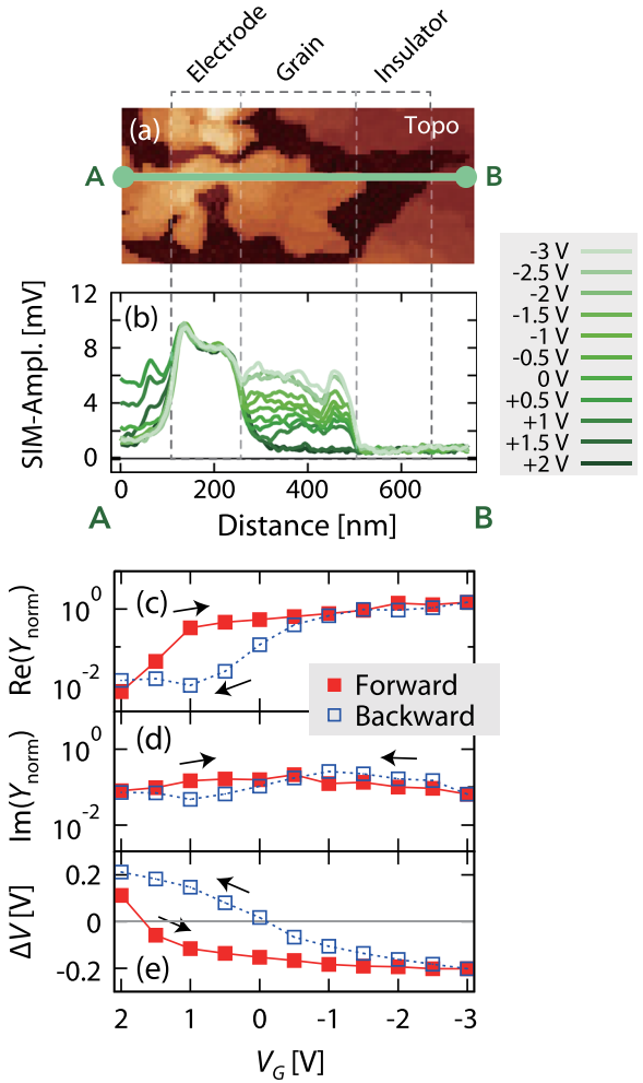
FIG. 6. (a) Topographic FM-AFM image of the area around the interface between the Pt electrode and grain A. (b) FM-SIM amplitude signal profiles measured along the A-B line indicated in (a). (c) and (d) The plots of the real part and imaginary part of the normalized interface admittance Y_{\text{norm}} as a function of V_G , respectively. (e) The plot of the potential drop across the interface \Delta V as a function of V_G . The solid symbols represent the data points measured during the forward sweep of V_G from +2 V to -3 V, and the open symbols represent the data points during the backward sweep.
