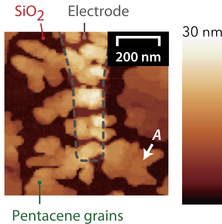
FIG. 3. Topographic image of pentacene grains near the metal electrode, which is enclosed by the dashed curve. The dark area surrounding the electrode and grains is the bare \text{SiO}_2 surface. Grain A indicated by the arrow is isolated from the other grains.
